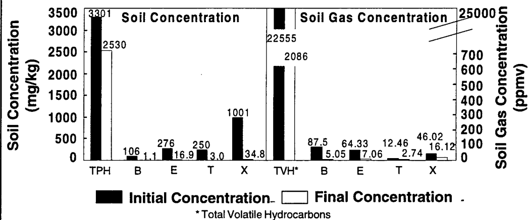
FIGURE 9. AVERAGE TPH AND BTEX CONCENTRATIONS: INITIAL AND 1-YEAR RESULTS
