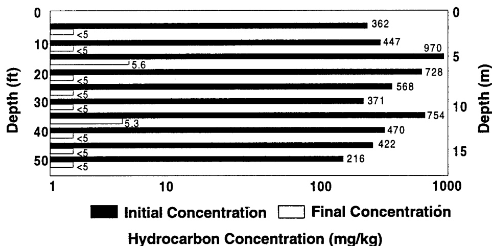
FIGURE 10. HILL AFB (BUILDING 914) SOIL SAMPLE RESULTS
