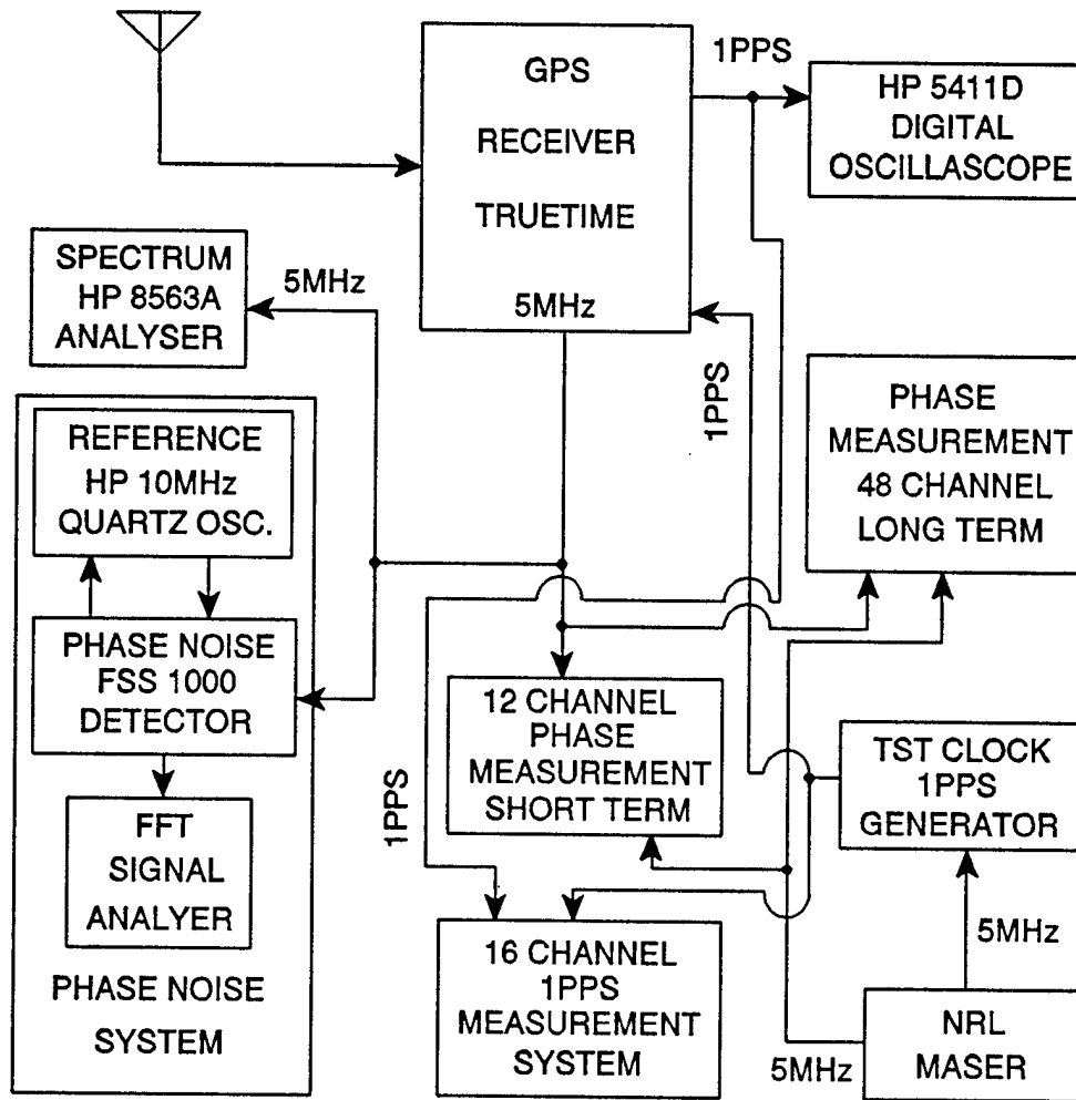
Diagram A.2. Precision clock evaluation facility.
