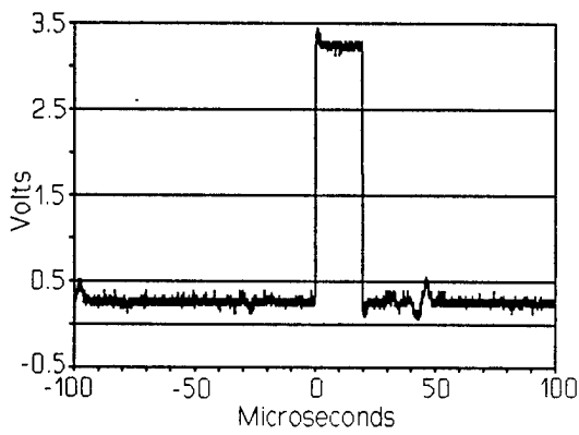
Figure D.2. 1PPS output.
