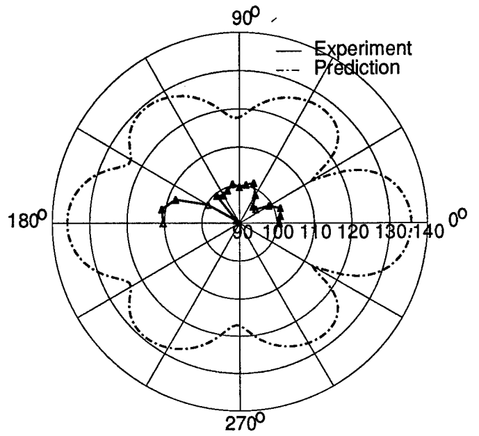
Figure B57: Test H1 - 3,5 Mode
