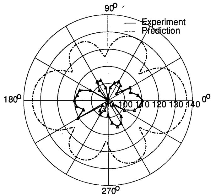
Figure B8: Test 3 - 3,5 Mode
