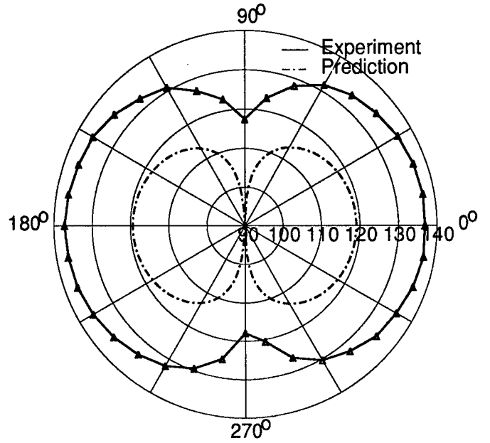
Figure A34: Test 8 - 1,1 Mode
