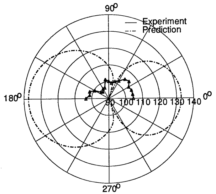
Figure B55: Test H1 - 4,1 Mode
