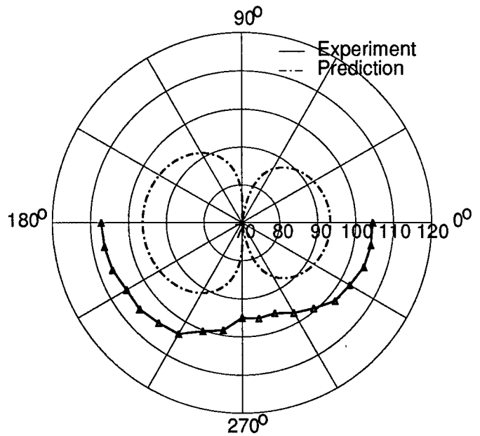
Figure A60: Test 12 - 250 Hz
