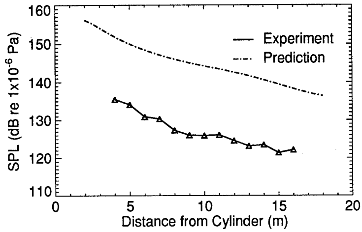
Figure B39: Test L1 - 2,3 Mode
