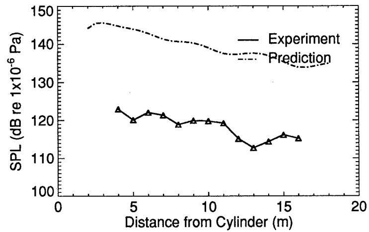
Figure B48: Test L2 - 3,5 Mode
