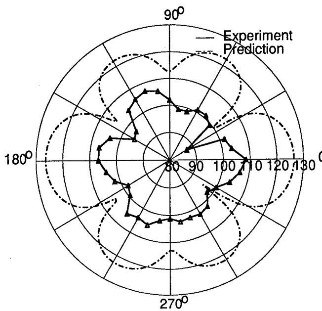
Figure B3: Test 3 - 3,1 Mode
