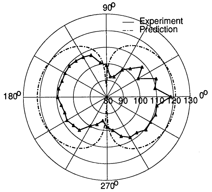
Figure B2: Test 3 - 1,1 Mode
