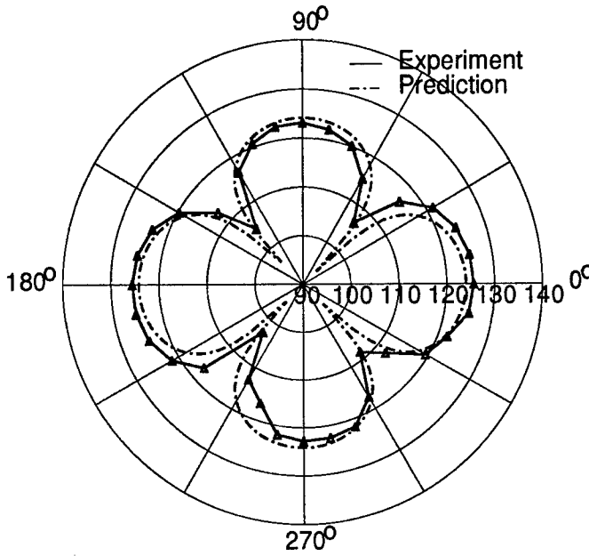
Figure A27: Test 7 - 2,1 Mode
