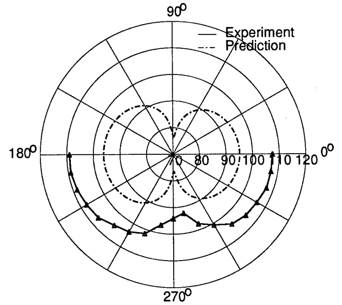
Figure A72: Test 14 - 250 Hz
