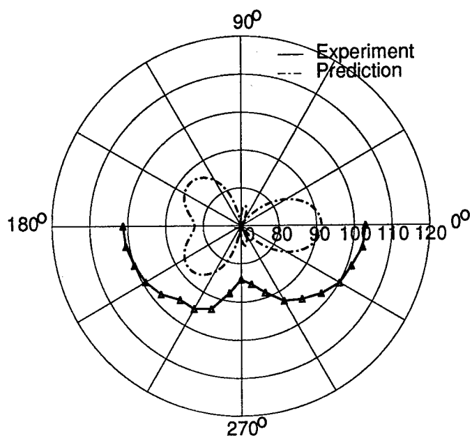
Figure A73: Test 14 - 400 Hz
