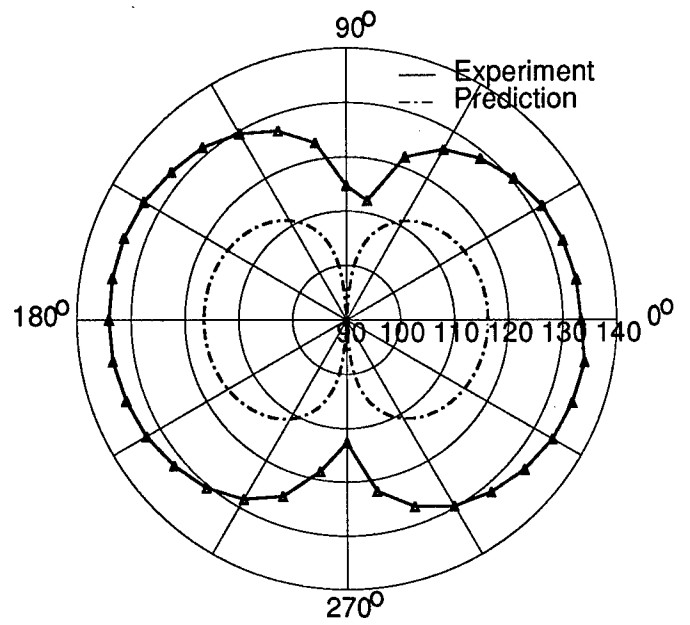
Figure A40: Test 9 - 1,1 Mode
