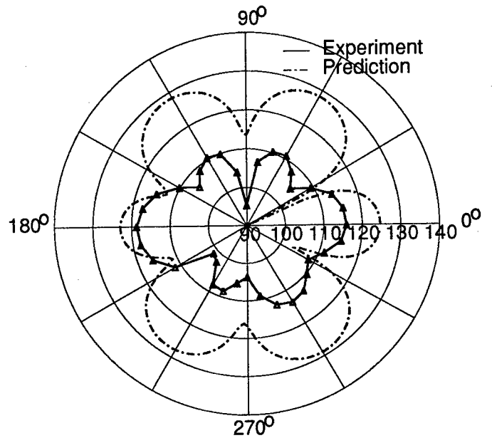
Figure A17: Test 4 - 3,3 Mode
