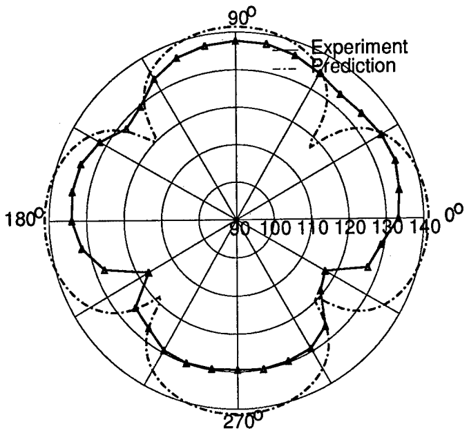
Figure A3: Test 1 - 2,3 Mode
