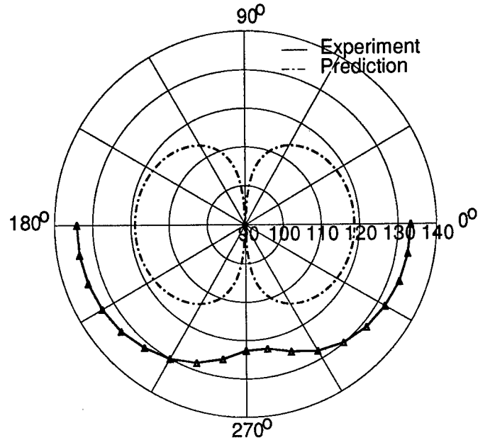
Figure A64: Test 13 - 1,1 Mode
