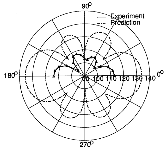
Figure B19: Test 6 - 3,5 Mode
