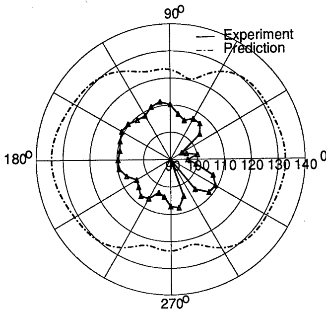
Figure A25: Test 6 - 4,1 Mode
