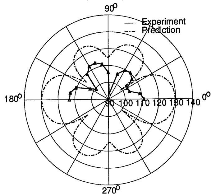
Figure B17: Test 6 - 3,1 Mode
