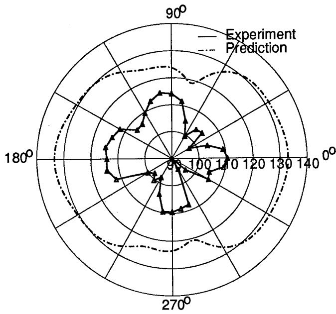
Figure A31: Test 7 - 4,1 Mode
