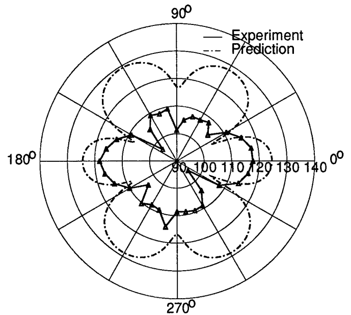
Figure A36: Test 8 - 3,3 Mode
