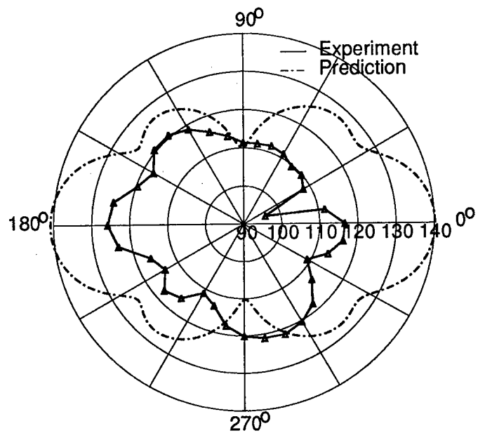
Figure A44: Test 9 - 3,5 Mode
