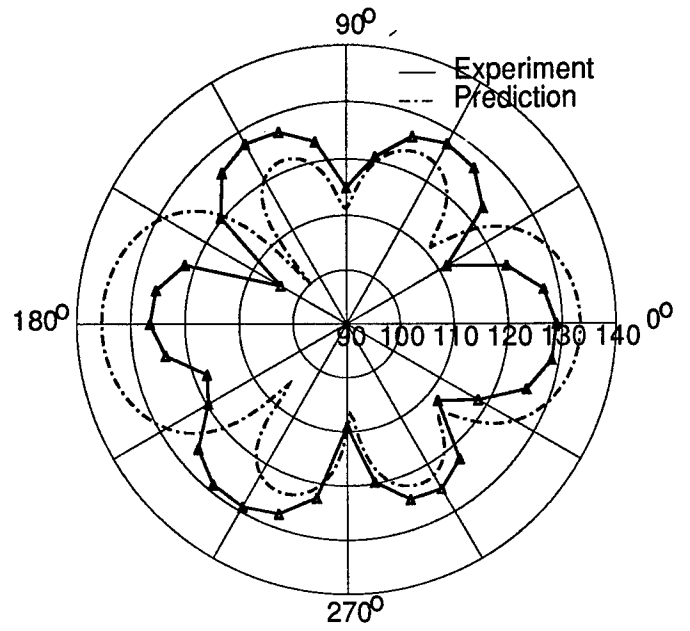
Figure A19: Test 4 - 3,5 Mode
