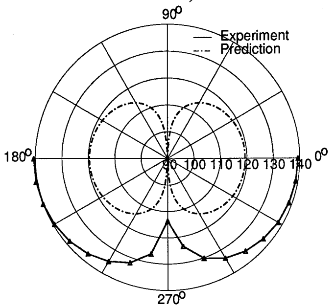
Figure A58: Test 12 - 1,1 Mode
