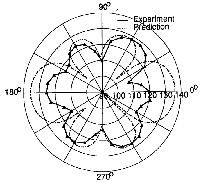
Figure A26: Test 6 - 3,5 Mode
