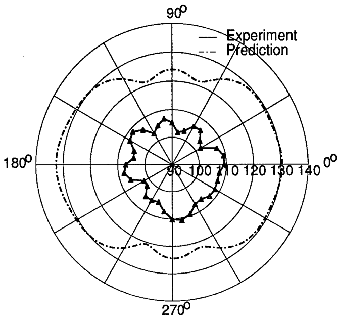
Figure A18: Test 4 - 4,1 Mode
