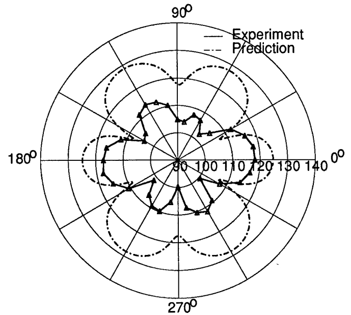
Figure A30: Test 7 - 3,3 Mode
