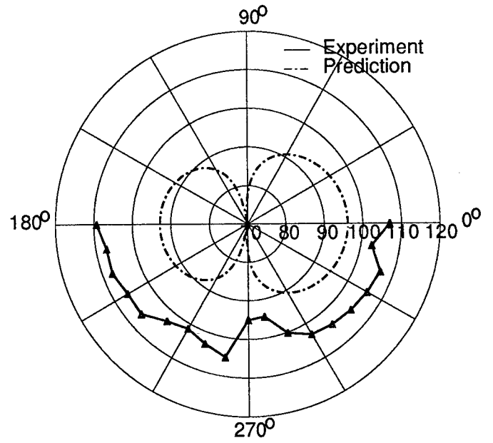
Figure A66: Test 13 - 250 Hz
