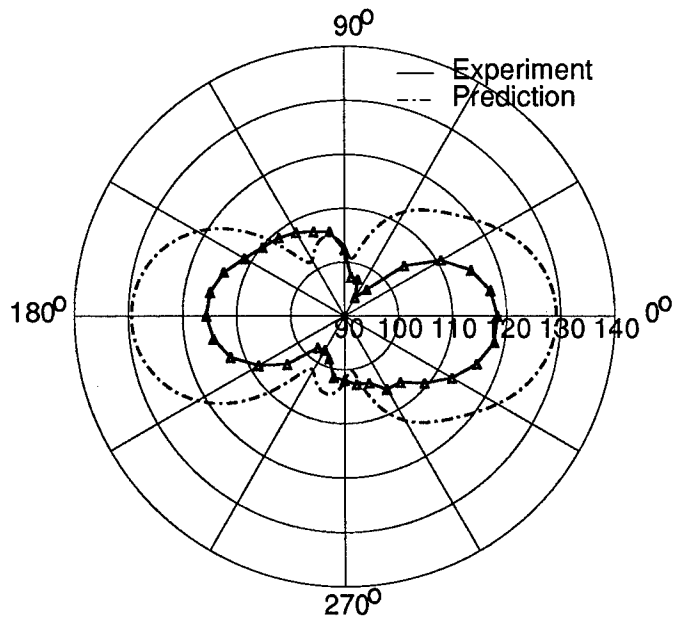
Figure A54: Test 11 - 3,3 Mode
