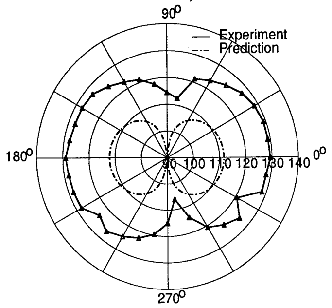
Figure A28: Test 7 - 1,1 Mode
