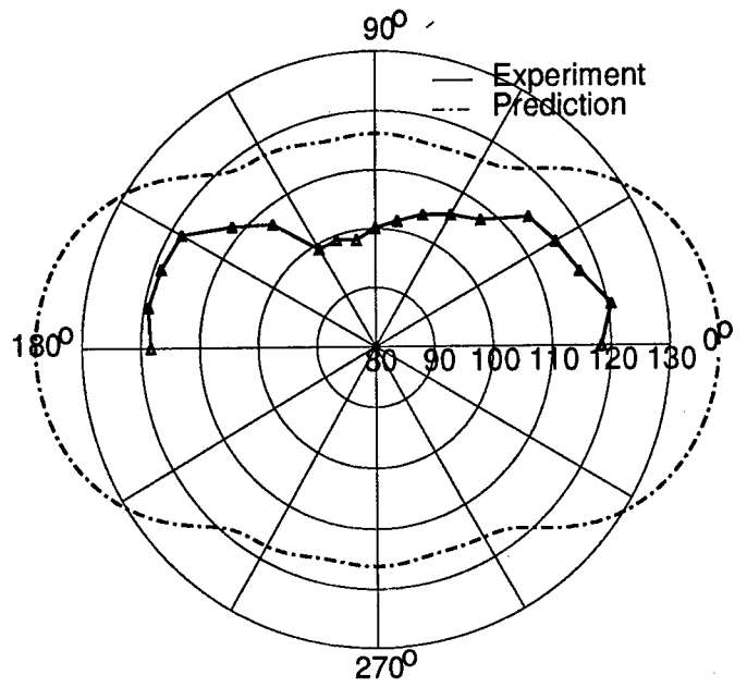
Figure B53: Test H1 - 2,3 Mode
