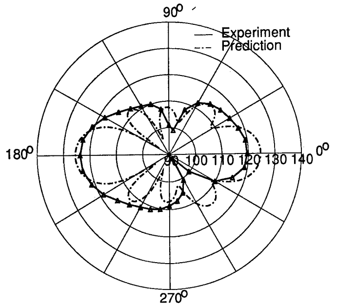
Figure A42: Test 9 - 3,3 Mode
