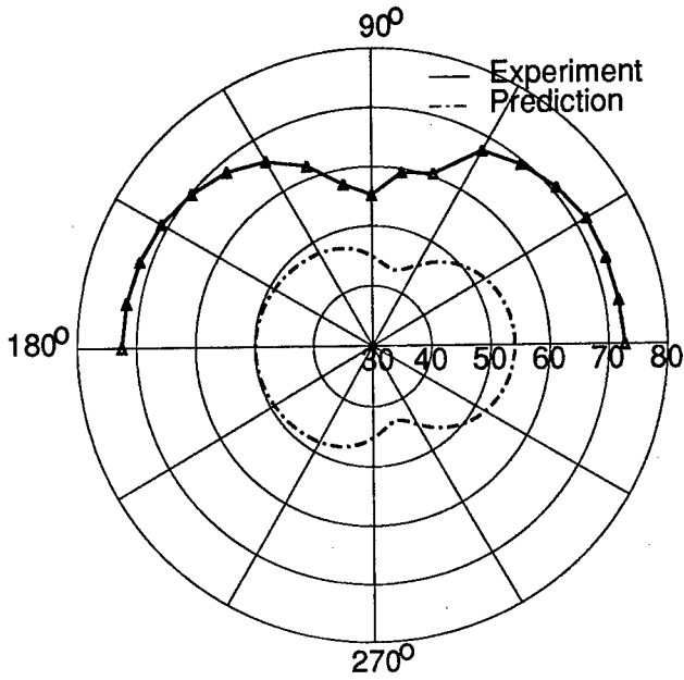
Figure B27: Test 8 - 50 Hz
