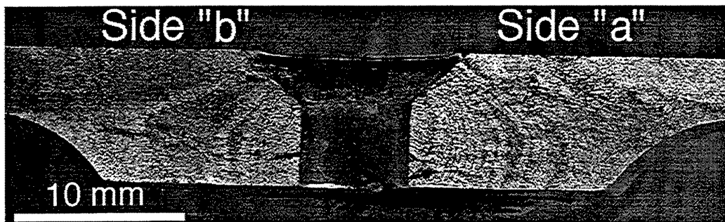
Figure 22. View onto fracture surface of first box specimen
