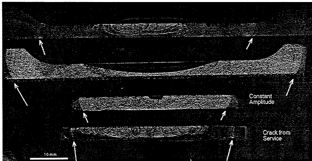
Figure 24. Fracture surfaces (from top down)
