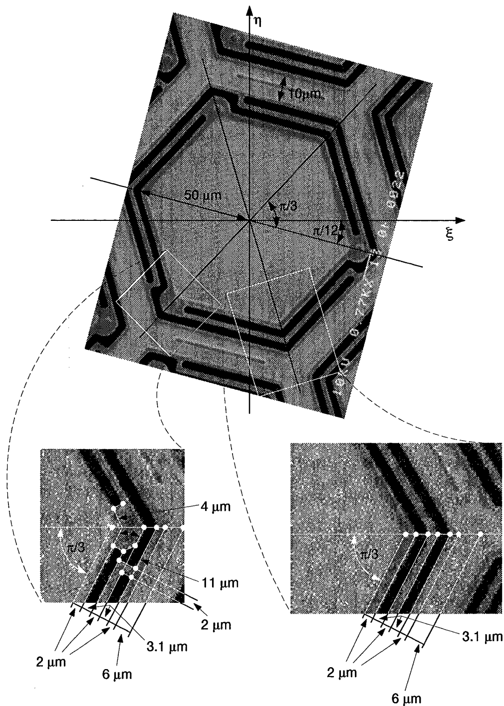
Figure 4. MUMPS9 geometry.
