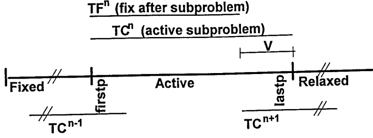
Figure 2. A single proximal cascade subproblem optimizes rows and columns indexed by the active set ( t \in TC^n ). Thus it re-optimizes rows and columns indexed by time periods active in the previous subproblem, t \in TC^{n-1} \cap TC^n . Rows of future time periods are relaxed, future columns are fixed at level 0. Columns of subproblem n that are not active in subproblem n+1 (indexed by t \in TF^n ) are fixed at the end of n .
