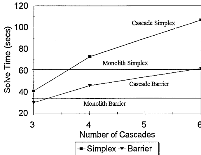
Figure 10. Large problems solve much faster using the barrier algorithm (IBM RS6000/590). The vertical axis shows the notional Southwest Asia cascade solution time in seconds; horizontal bands represent the monolith solution time. The horizontal axis shows the number of subproblems, which is a function of cascade width, caswid , and cascade overlap, v . The plots represent the simplex and barrier times with caswid fixed at 15, and v = 5, 10, and 12. These parameter settings specify the number of subproblems to be 3, 4, and 6, respectively.
