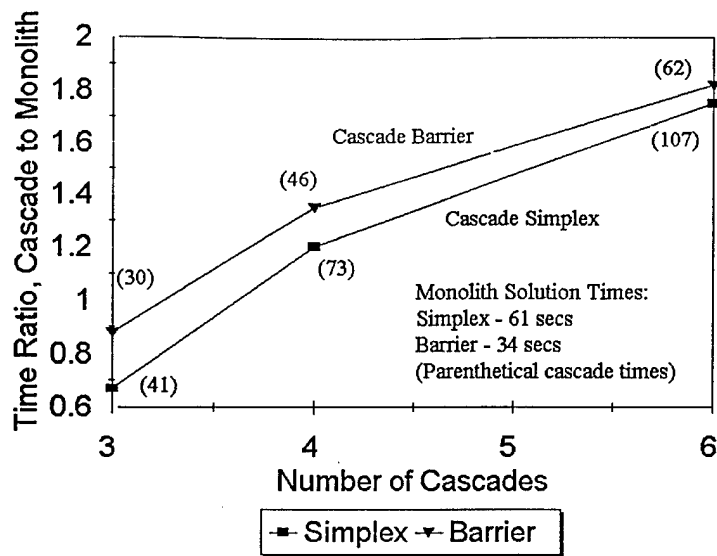
Figure 11. This plot includes the same data as in the previous figure (Notional Southwest Asia, caswid =15), but the vertical axis depicts the solve times as a ratio of the cascade solution to the monolith solution. Because the simplex ratios are lower than the barrier ratios, this figure shows that simplex cascades perform better than barrier cascades when compared to their respective monolith solution times.
