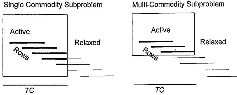
Figure 3. Unlike its single commodity counterpart, a multi-commodity proximal cascade subproblem excludes both columns and rows indexed by future time periods. These rows are required only for the segmented results of the previous section, and may cause infeasibility in more general problems.
