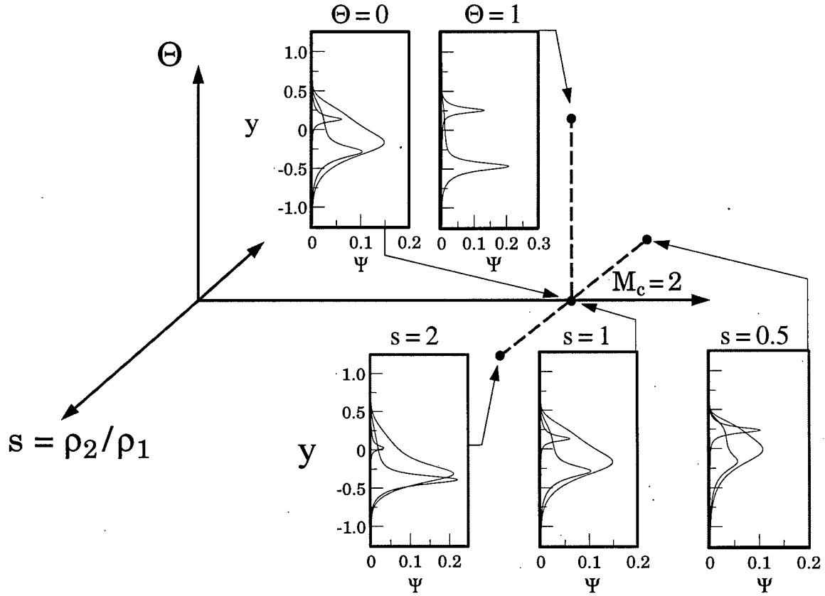
Fig. 5: Effect of heat release and density ratio variation on the amplification rate normalized eigenfunction energy profiles at high compressibility ( M_c = 2, \phi = 1, \bar{u}_2 = 0 ).
