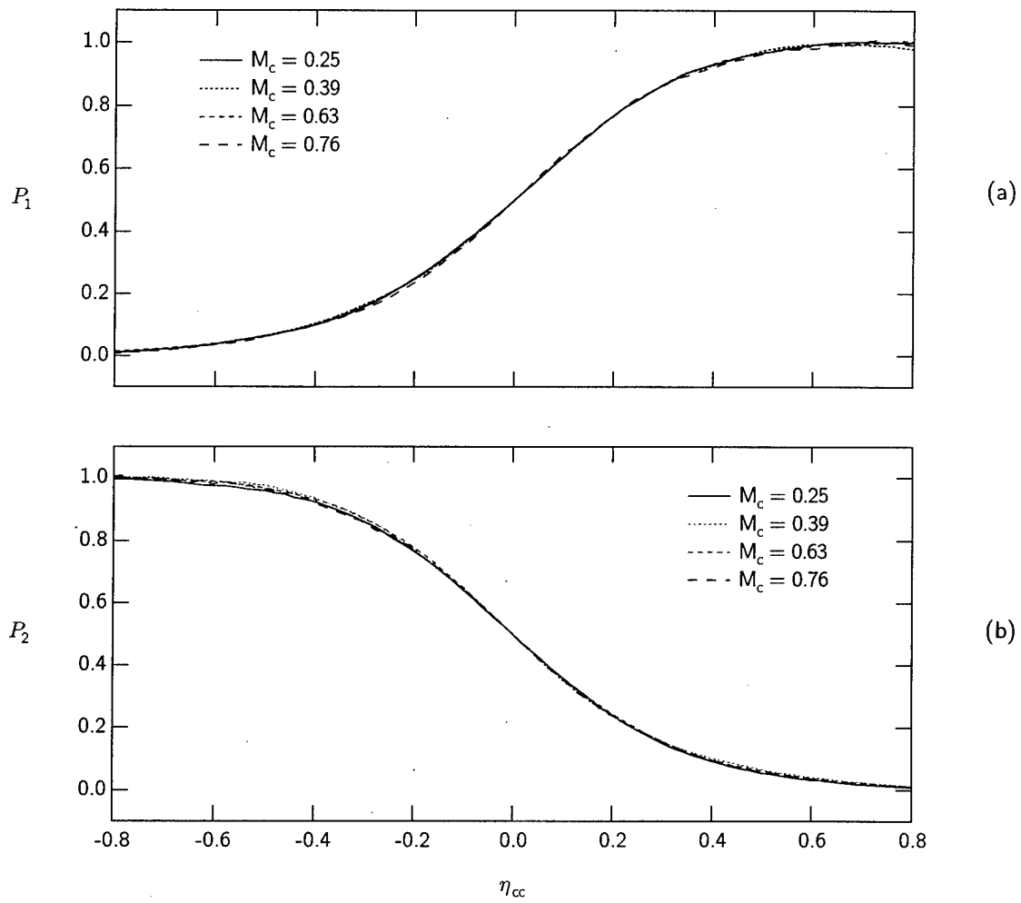
Fig. 18. Re -averaged pure fluid profiles obtained with the cold chemistry method. The transverse coordinate \eta_{cc} is scaled on the cold chemistry data itself.
