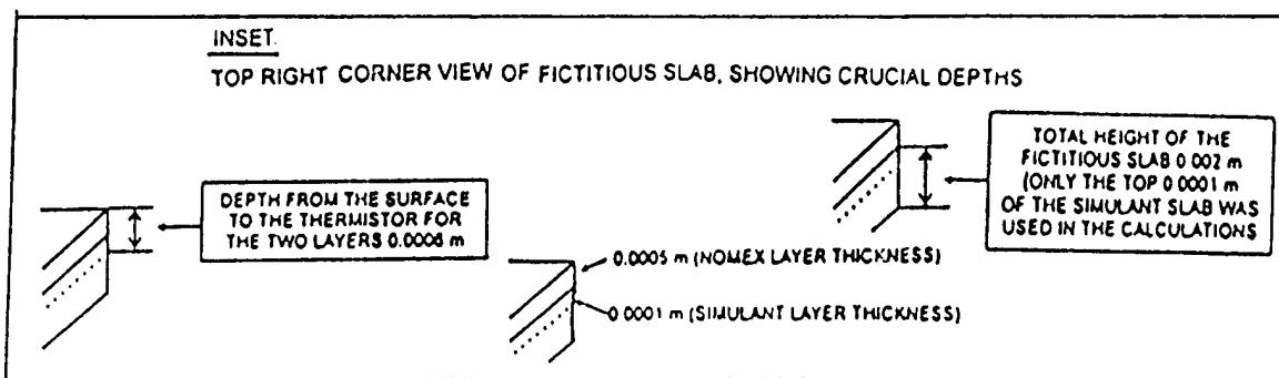
FIGURE 1(c). SKIN SIMULANT AND NOMEX COMPUTER INPUT--TWO LAYERS
