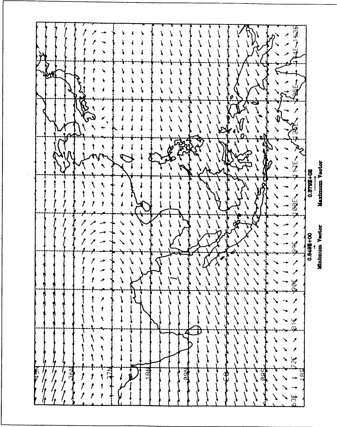
Figure 16. Average 200 hPa Winds (m/s) for August, 1991.
