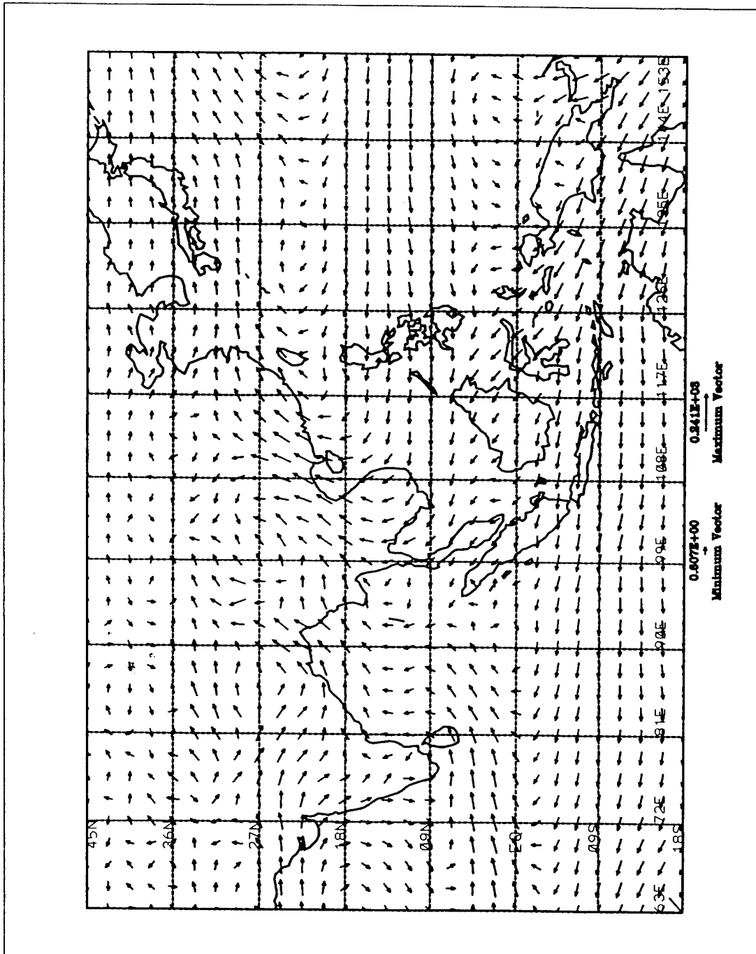
Figure 24. Average Horizontal Moisture Flux at 850 hPa (g/kg m/s) for May, 1991.
