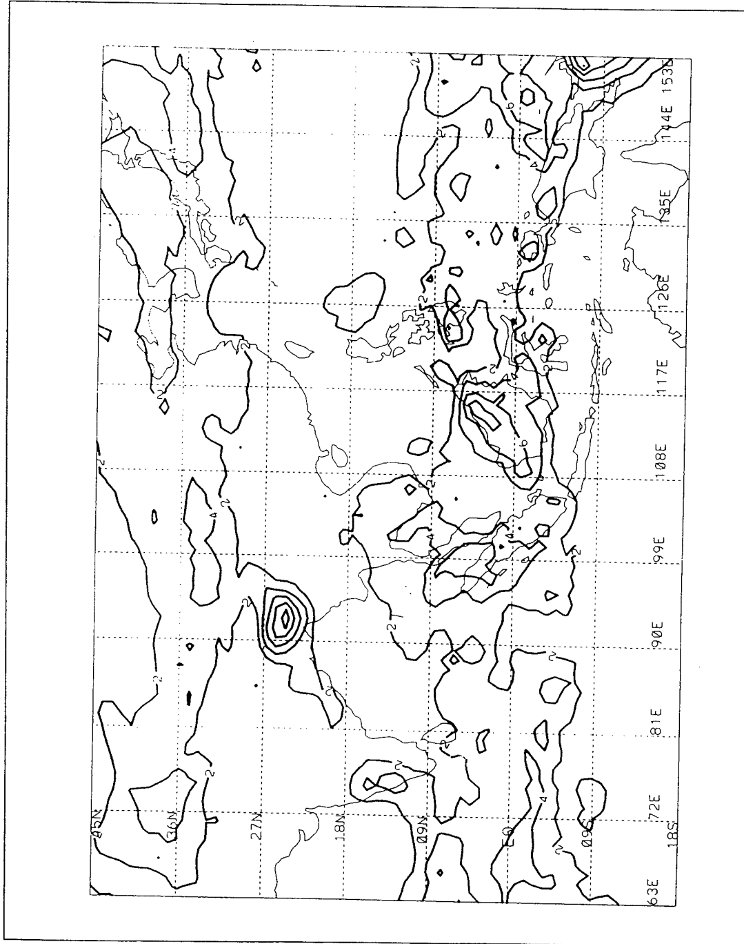
Figure 1. Average Convective Index (CI) for May, 1991. Values of CI are in °K.
