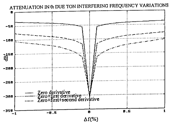
Figure 5. Attenuation in \theta_f when changes affect the interfering frequency. 0% means the interfering frequency has not been affected.
