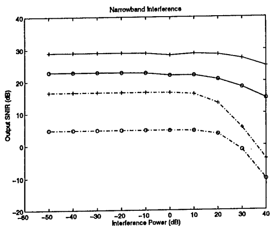
Fig. 2: Output SNIR with narrowband jamming
