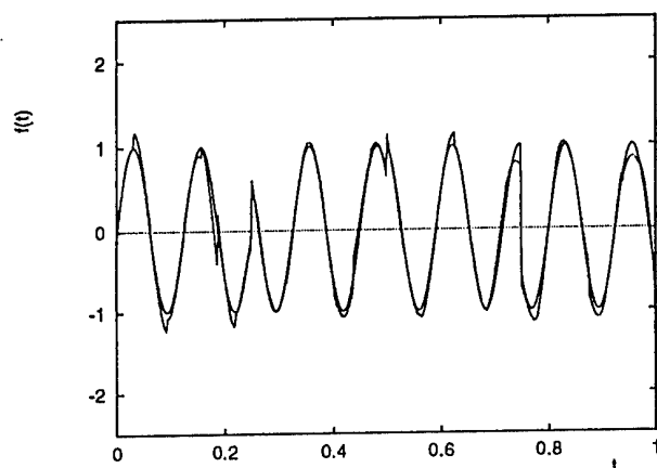
Figure 7: The continuous curve plots the original signal. The dotted line plots the reconstruction obtained through both, the wavelet and orthonormal representations.
