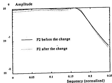
Figure 10: F2 before and after the change.
