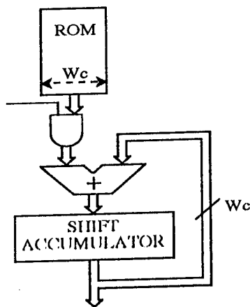
Figure 4: Architecture of the quantizer
