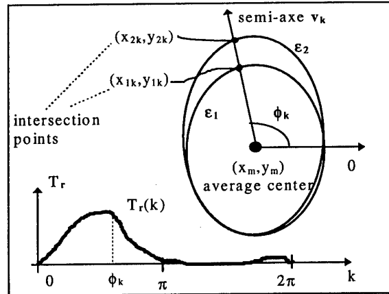
Figure 4. The similitude trace T_r of the two ellipses e_1 and e_2 is drawn for 0 < k < 127 . For a given semi-axis v_k the intersection points (x_{1k}, y_{1k}) (x_{2k}, y_{2k}) and the value of T_r(k) are outlined.
