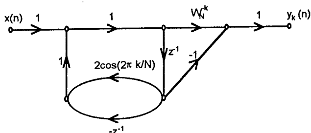
Figure 1. Goertzel algorithm
