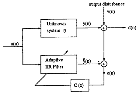
Figure 1: System Identification Configuration
