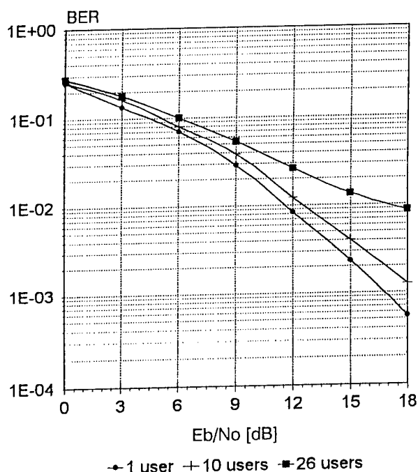
Fig. 5 The performance of the adaptive correlator receiver in the presence of intracell interference
