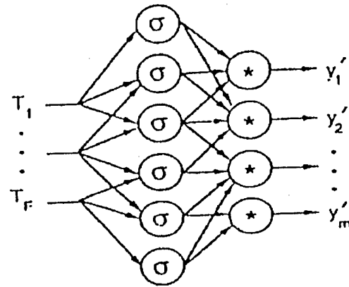
Figure 2: The decoding phase of the NLPCA network.
