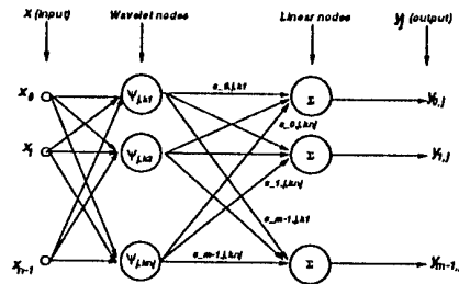
Fig. 2. The wavelet network at scale j
