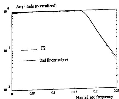
Figure 5: Frequency response of F2 and the NN model.
