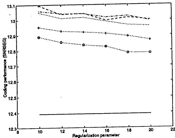
Figure 3: Coding performance vs. regularization parameter for different nonlinear analysis frame lengths (in samples): 100 (— —), 80 (— · —), 60 (····), 40 (· · + · ·), and 20 (····).
