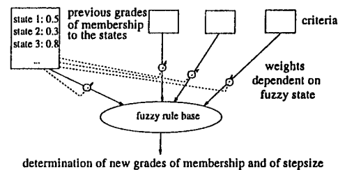
Figure 3: Concept for the logic of the control unit, fuzzy states. Dashed lines mark weight control.
