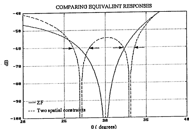
Figure 8. Linear array with an interferer in \theta_i=30^\circ . ZF case vs. response with spatial constraints in \theta_1=27^\circ and \theta_2=33^\circ .
