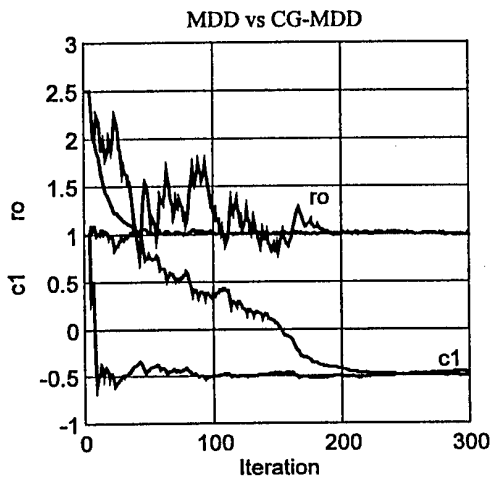
Fig.3. Evolution of the coefficients of the instantaneous gradient and conjugate gradient algorithms.
