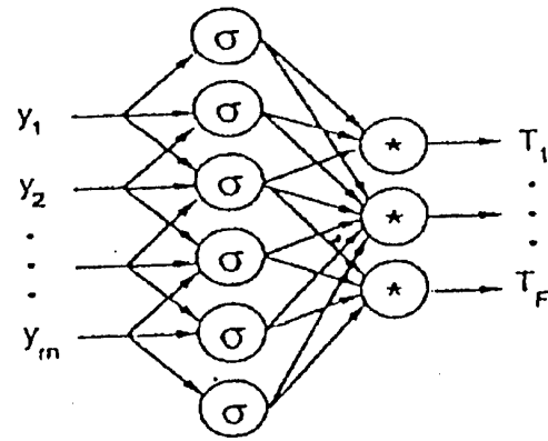
Figure 1: The encoding phase of the NLPCA network.
