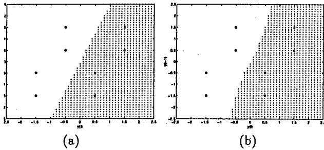
Figure 2: Decision regions formed by the LRE equalizer or H(z) = 1 + 0.5z^{-1} for (a) 21 dB and (b) 11 dB SNR. "x" represents x_n = 1 and "o" x_n = -1 .
