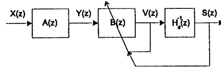
Figure 1: Feed-forward structure.
