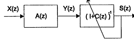
Figure 2: Feed-Backward structure.
