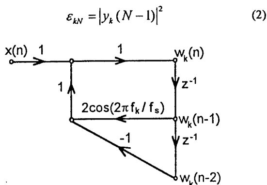
Figure 2. Goertzel algorithm for DTMF signal detection
