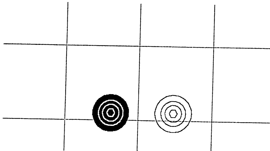
Figure 14. Vortex evolution in a stratified shear flow with Ri = 1.0 . Laboratory streak photographs (top) and total streamfunction (middle) and perturbation vorticity (bottom) plots from a numerical simulation are shown for nondimensional times of (a) 0.10, (b) 0.36, (c) 0.62, and (d) 0.76. Horizontal and vertical grid separation is 10 cm.
