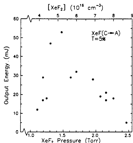
Fig. 3. Dependence of C \rightarrow A laser output pulse energy on the \text{XeF}_2 partial pressure for a 600-Torr Ar/190-Torr \text{N}_2 /6-Torr \text{SF}_6 gas mixture at 300 K.
