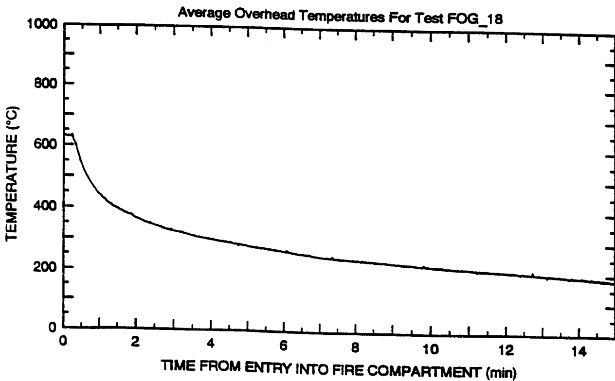
Fig. 24 - Wood crib and average overhead temperatures for FOG_18
