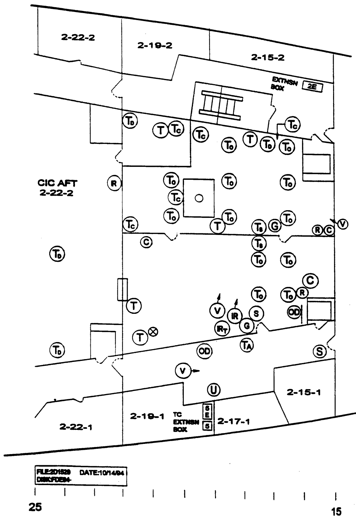
Fig. A4 - Second deck instrumentation layout
