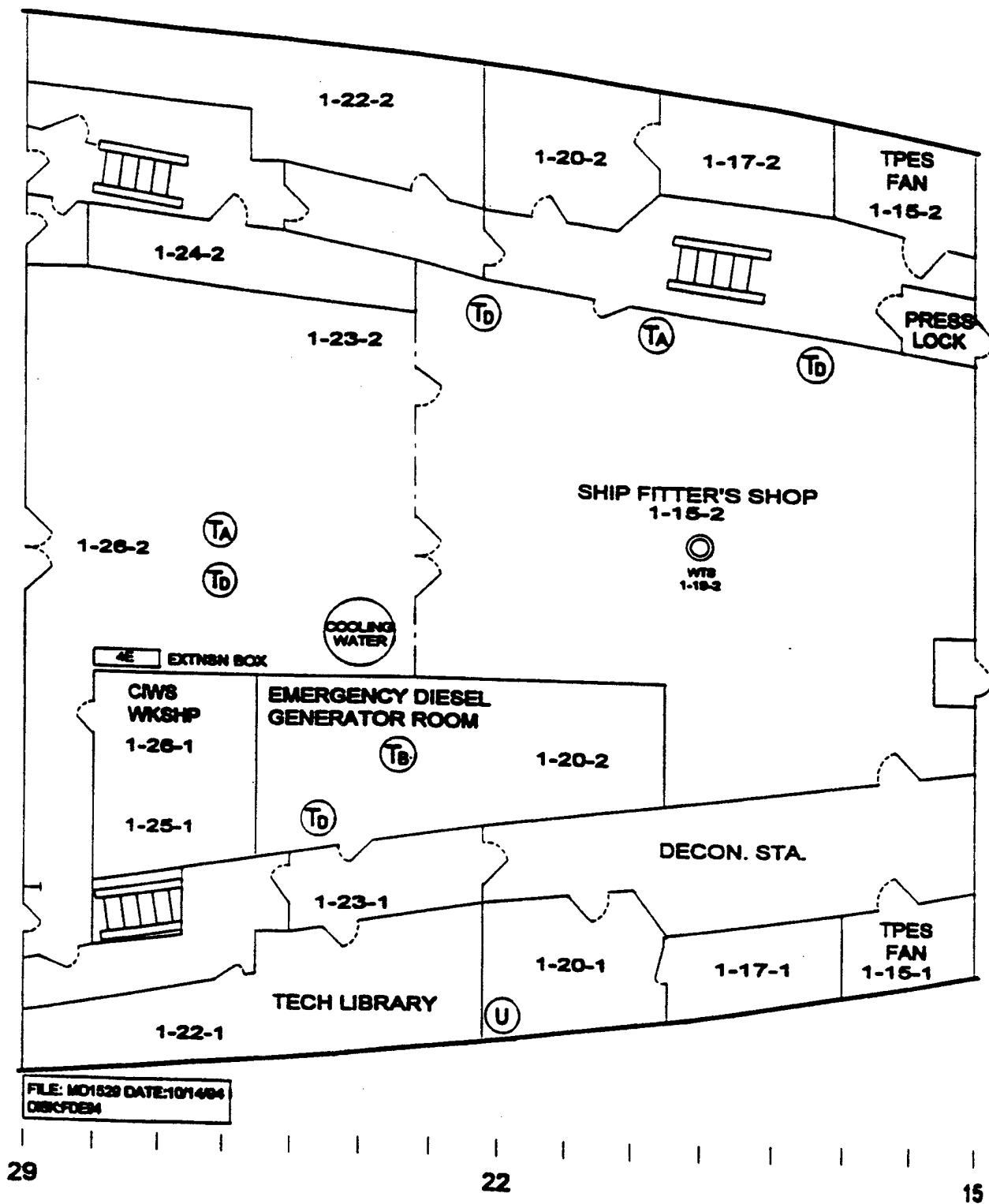
Fig. A3 - First (Main) deck instrumentation layout
