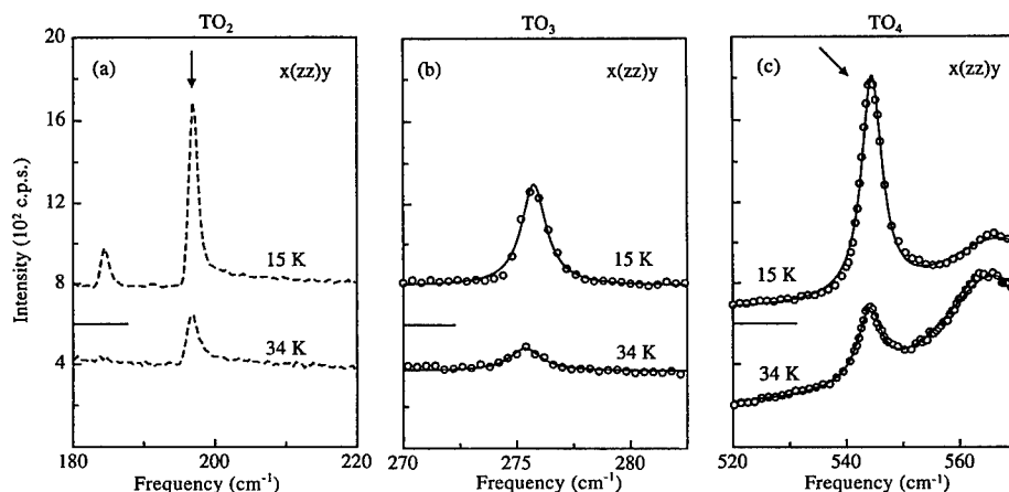
FIGURE 1 ZFC Raman spectra from \text{TO}_2 , \text{TO}_3 , \text{TO}_4 hard phonons, above and below the transition temperature ( T_i = 32 K) in \text{KTa}_{0.976}\text{Nb}_{0.024}\text{O}_3 . Full lines denote Lorentzian fits to the experimental data.
