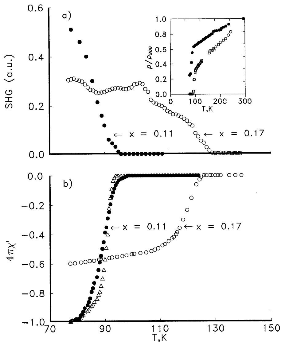
FIGURE 1 Temperature dependence SHG (a) and AC- magnetic susceptibilities (b) for Hg-1201: \Delta -after the syntheses, \bullet -after the annealing in flowing O_2 at 350^\circ C (8h), \circ -after the reannealing in flowing O_2 at 600^\circ C (2h).
