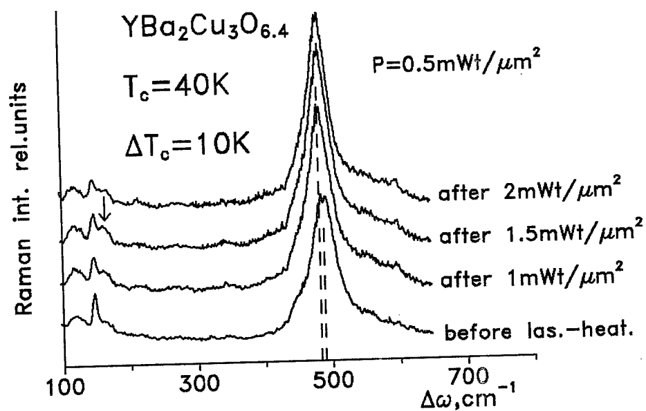
FIGURE 2 Raman spectra of the YBa 2 Cu 3 O 6.4 single crystal ( P = 0.5 \text{ mW}/\mu\text{m}^2 ) measured after laser-heating with different pump power.
