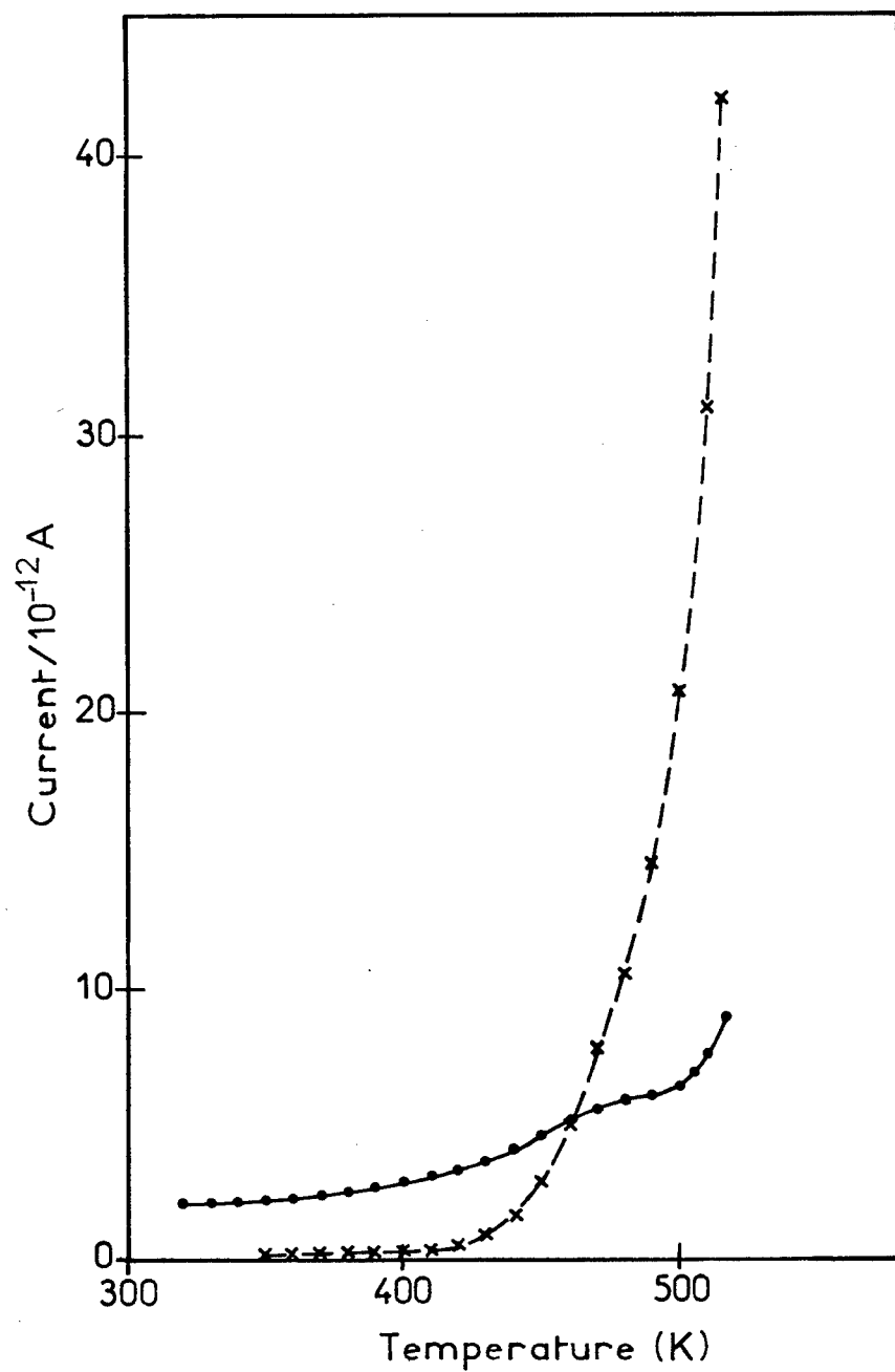
FIGURE 1 Thermostimulated electric current of silica samples : \times glass sample (Suprasil 1), \bullet crystalline quartz. The heating rate temperature is: 0.2 K/s.
