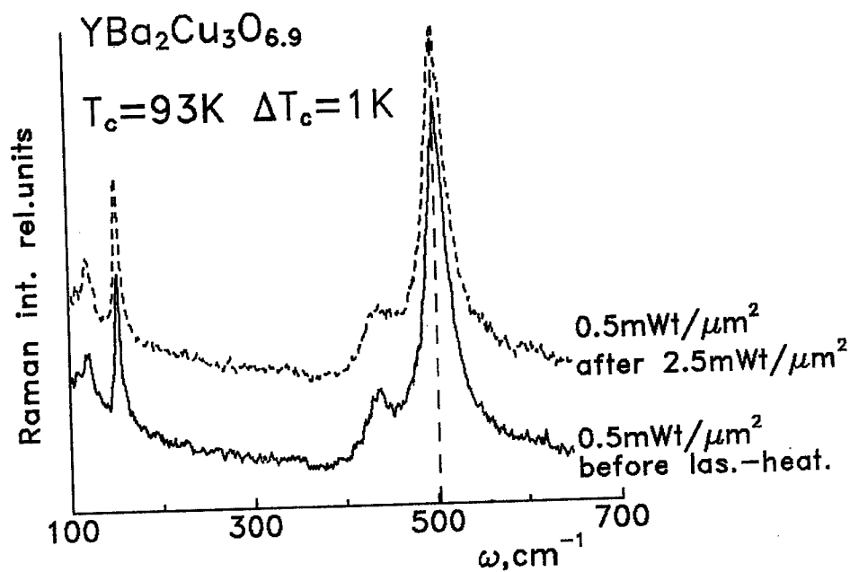
FIGURE 1 Raman spectra before (1) and after (2) laser-heating \sim 2.5 \text{ mW}/\mu\text{m}^2 in the YBa 2 Cu 3 O 6.9 single crystal.
