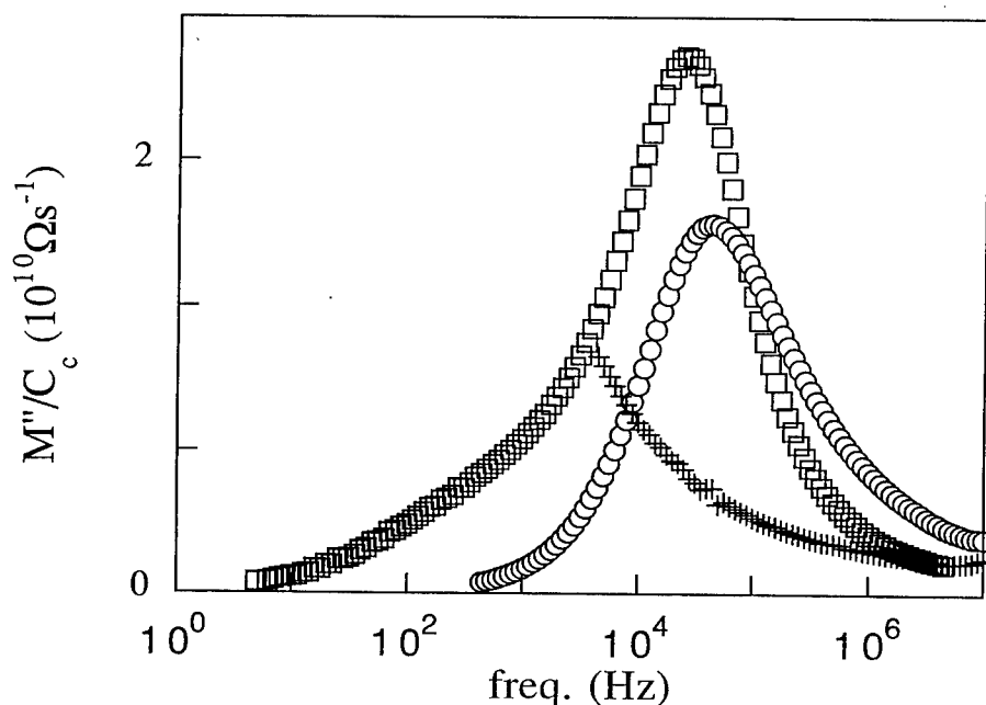
FIGURE 1 Imaginary part of the complex modulus (divided by the capacitance of the empty holder) versus frequency of a thermochemically reduced sample: \square after reduction measured at 270°C, \times after a partial reoxidation at 420°C (measured at 270°C), and \circ reoxidized sample measured at 415°C.
