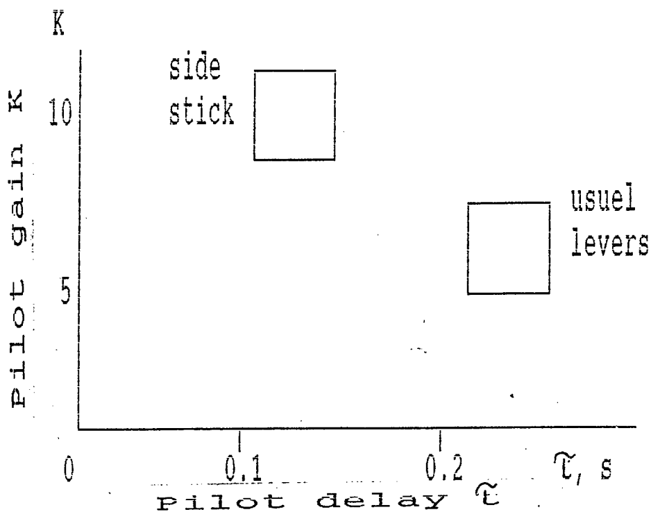
Fig.2.4. Lever type influencing on dynamic properties of a pilot
