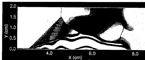
When a shock propagates down a tube, it creates a boundary layer at the wall. When this shock reflects from the end wall, back into the boundary layer, a complex lambda shock structure may develop. This figure shows pressure contours for a computation on the CM-5 of a reflected shock (moving from the right, to the left) propagating into a boundary layer. The light area on the left side is the once-shocked material, in which there is a small boundary layer near the wall. The complex structure that results contains many shocks and shear layers. Near the end wall, the material has a high temperature and essentially zero velocity.
