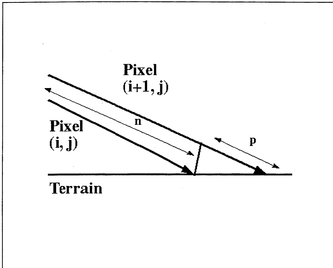
Figure 1.4. Zig-Zag Feature of Ray Trace. After Ref.[1].
