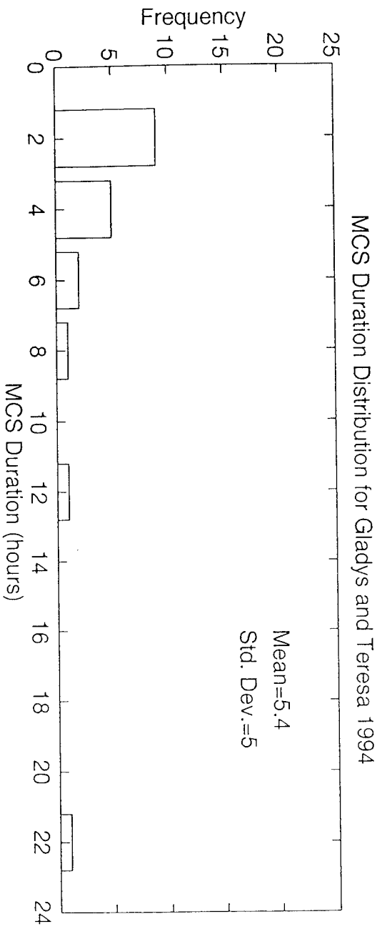
Fig. 5.C.3 MCS size and duration distributions for Typhoons Gladys and Teresa, 1994.
