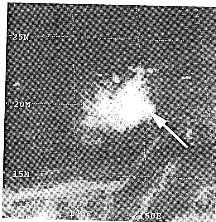
Fig 3.B.3 As in Fig. 3.B.2, except at 06 UTC 13 August 1994. Arrow indicates developing MCS.
