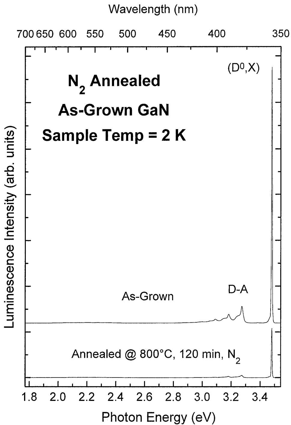
Figure 5-12. Photoluminescence spectra taken at 2 K for as-grown GaN and GaN annealed at 800 °C for 120 min in a N 2 environment.
