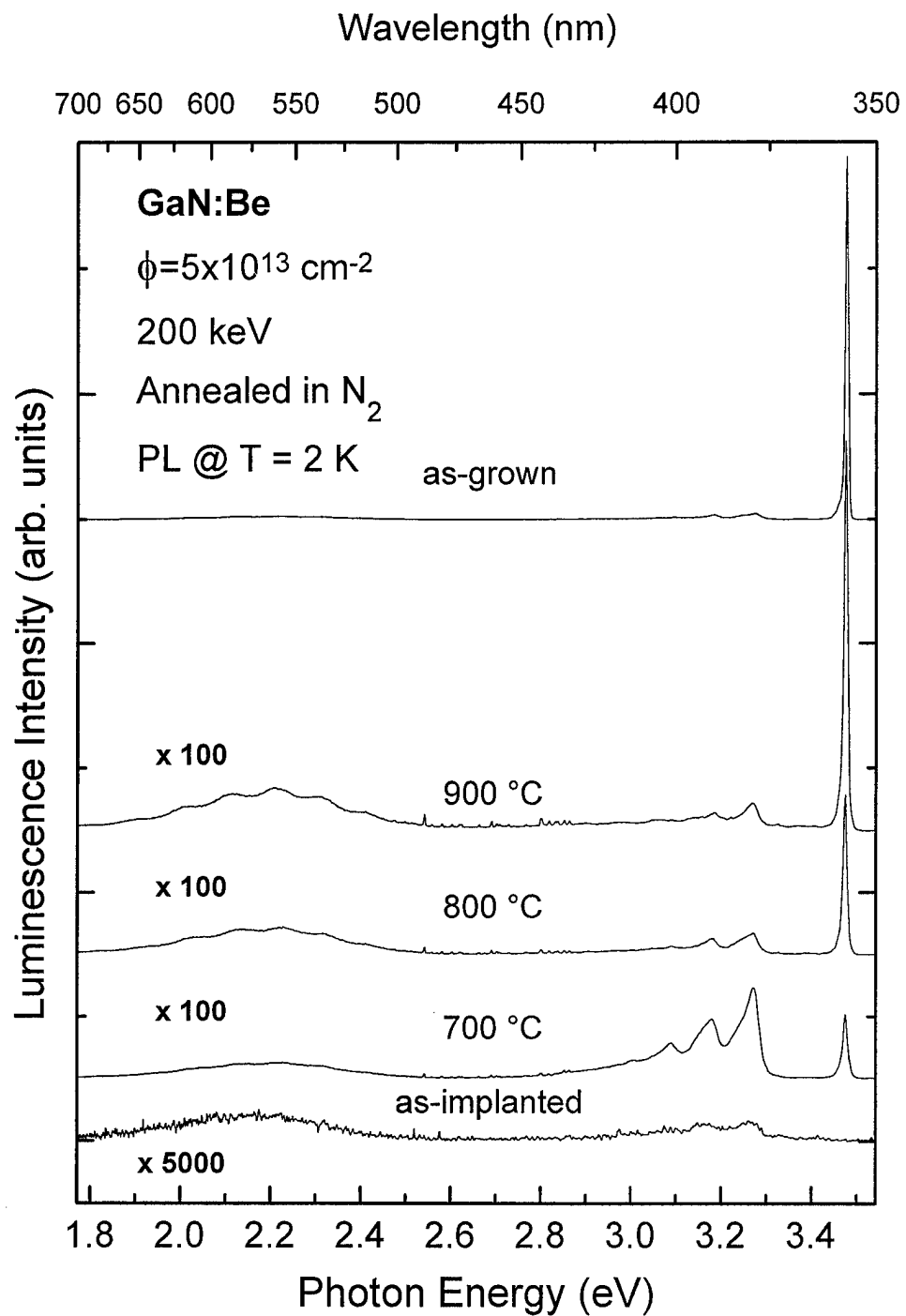
Figure 5-43. Photoluminescence spectra at 2 K of GaN implanted with beryllium at 200 keV to a dose of 5 \times 10^{13} \text{ cm}^{-2} and annealed at various temperatures in \text{N}_2 along with as-grown GaN spectrum.
