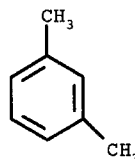
M-Xylene
