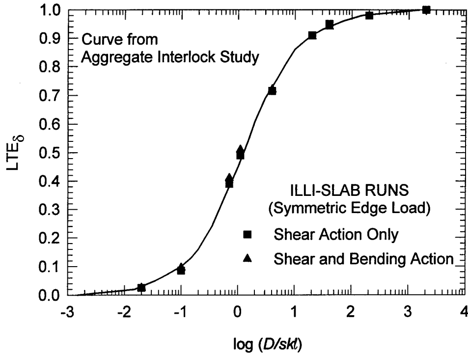
FIGURE 11. JOINT EFFICIENCY AS A FUNCTION OF DIMENSIONLESS JOINT STIFFNESS FOR DOWELED JOINT (AFTER IOANNIDES AND KOROVESIS, 1992)
