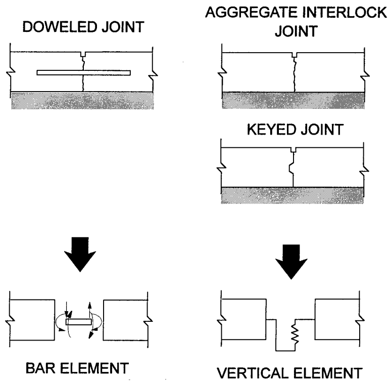
FIGURE 9. ILLI-SLAB JOINT MODEL (AFTER LARRALDE AND CHEN, 1985)
