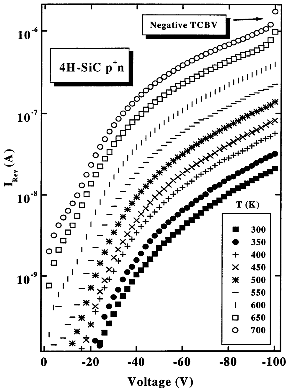
Figure VIII-19. Reverse-bias I-V-T series of data sets for a diode with a forward-bias shunting characteristic. The 4H-SiC p + /n diode curves shown correspond to measurement temperatures from 300 to 700 K. A dominant feature of the reverse characteristics of these diodes is illustrated by the 650 and 700 K curves showing initiation of reverse breakdown at 95 volts. This negative temperature coefficient of breakdown voltage was pervasive throughout the range of devices tested.
