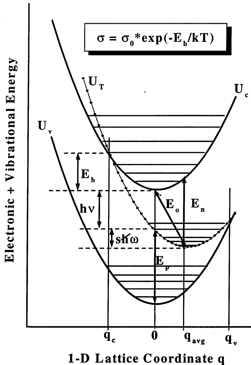
Figure III-5. Configuration coordinate diagram for a deep trapping level illustrating the origin of the exponentially varying capture cross section \sigma(T) . Included are the optical excitation threshold before ( E_p ) and after ( E_n ) relaxation, total binding energy ( E_0 ), lattice relaxation increase in binding energy ( s\hbar\omega ) after relaxation, and the thermal capture barrier ( E_b ). The average trap coordinate position ( q_{av} ) and the peak vibrational positions when the trap level crosses into the conduction ( q_c ) and valence ( q_v ) bands are also indicated.
