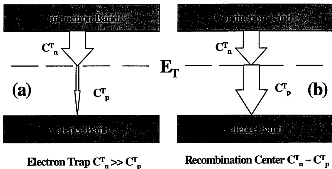
Figure III-2. Graphical representation of the differences between (a) traps and (b) recombination centers as related to a deep level bandgap state designated by the dashed line and label E_T . The arrow directions denote the loss of electron energy as trapping and recombination occurs. The arrow size relates to the magnitude of the capture rate.
