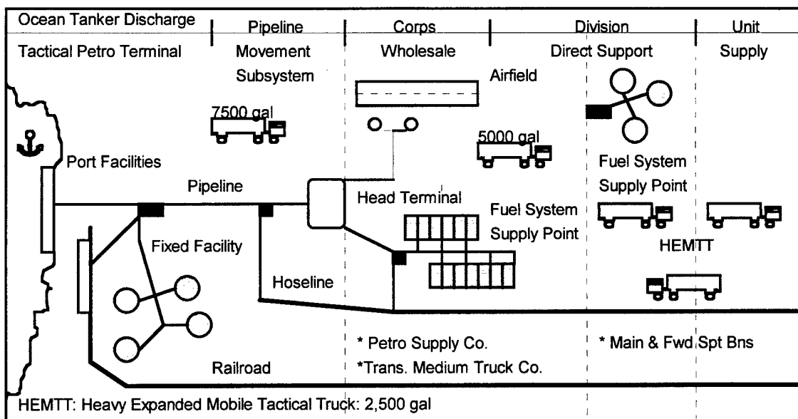
Figure 1. Bulk Petroleum Distribution System in a Developed Theater Source: Joint Publication 4-03. Joint Petroleum Doctrine
