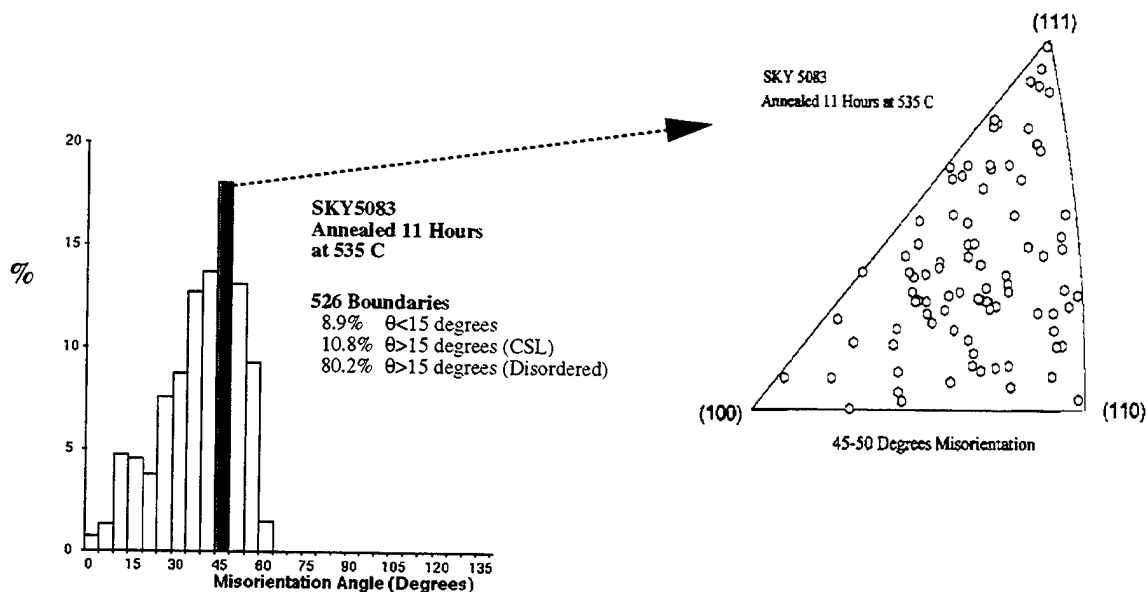
Figure 7.4. Boundary misorientation angle graphs and grain misorientation texture plots for (a) as-processed and (b) processed and annealed specimens. GMT plots are shown for the misorientation range where the peak fraction of boundaries was observed. There is a shift upward in this range with prolonged annealing. The GMT plots illustrate that the boundaries are primarily disordered.
