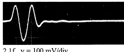
2.1f y = 100 \text{ mV/div.} x = 500 \text{ pSec/0.85 div.}
