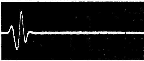
2.2d y = 50 \text{ mV/div.} x = 500 \text{ pSec/0.85 div.}
