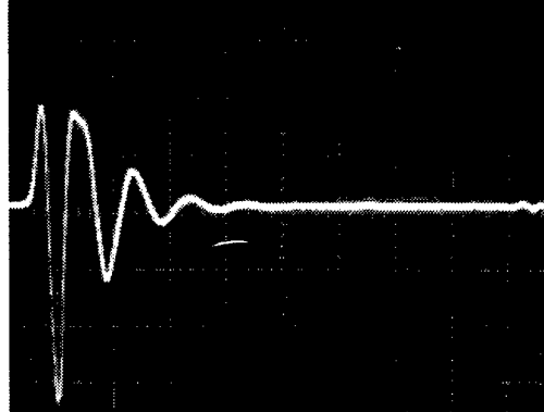
6.1b Butterfly y = 0.1 \text{ V/div.} x = 500 \text{ pSec/0.85 div.}
