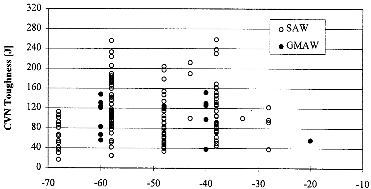
Figure 4.52: Average CVN toughness of weld metals deposited using the submerged arc and gas metal arc welding processes (data for submerged arc welds shown at a temperature 2°C higher than the actual test temperature)
