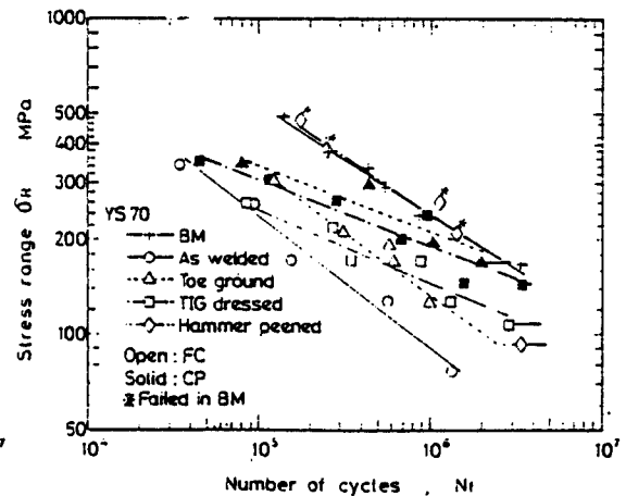
Effect of weld toe treatment on the fatigue strength of the YS70 steel in the artificial sea water
