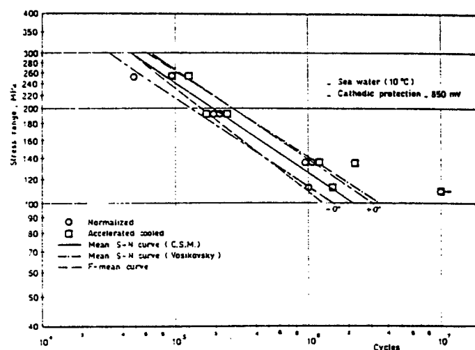
Results from T-butt tests in sea water with cathodic protection
