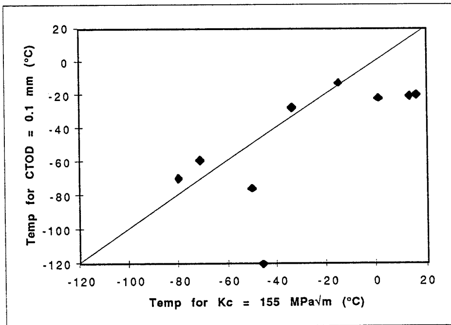
Figure 4.50: Data for machined notched centre cracked wide plate tests for fusion line (HAZ). CTOD temperature determined from lower bound of reported data (limited tests), T(155) found from regression \ln K_c against 1/T^\circ\text{K}
