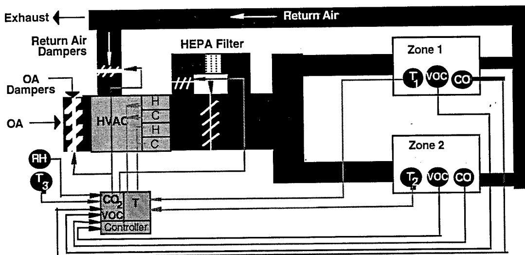
Figure 4. Filter By-Pass IAQ Control.
