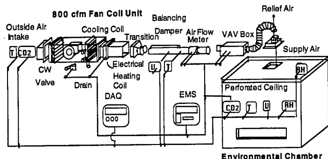
FIG. 2. Experimental Setup
