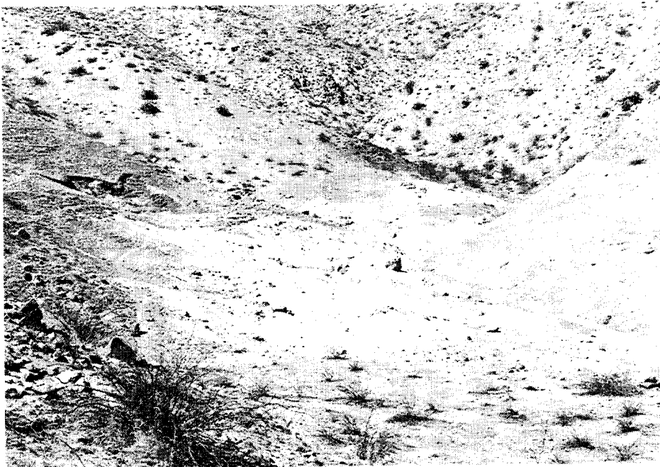
FIGURE 11. Northern West Canyon Land Slump, October 1996.
