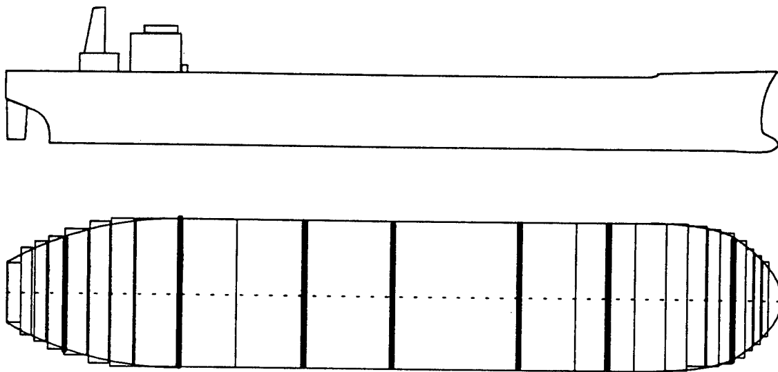
Figure 3.3: Division of a vessel into transverse sections
