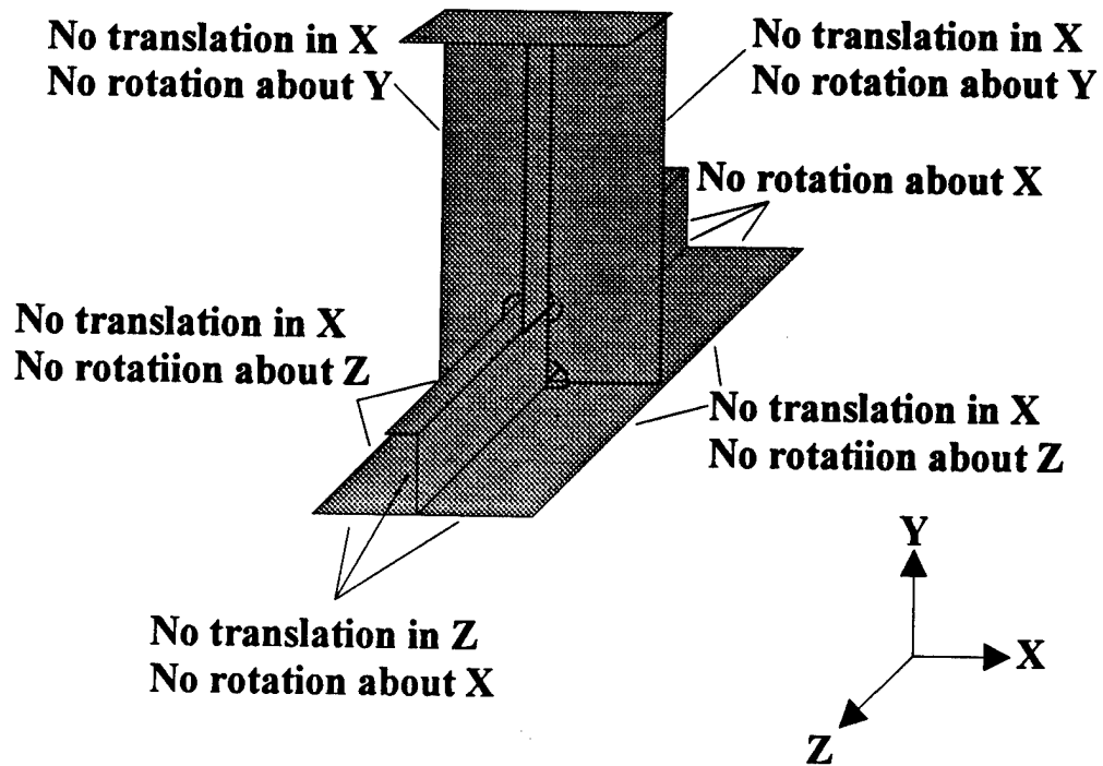
Figure 5.2: Boundary condition
