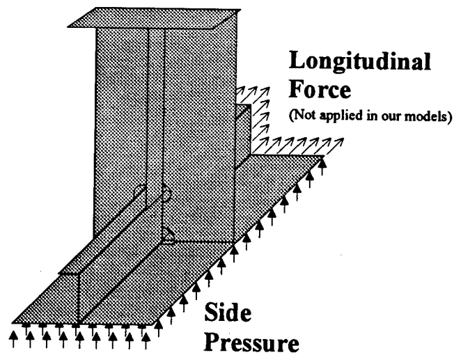
Figure 5.3: Load condition
