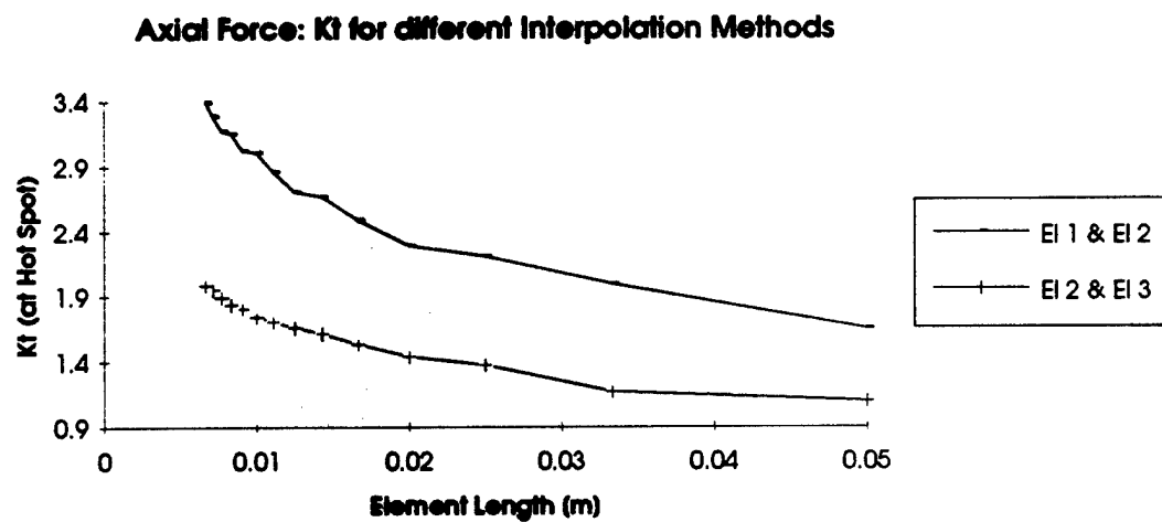
Figure 3.41: K_t for different Extrapolations: Axial Force
