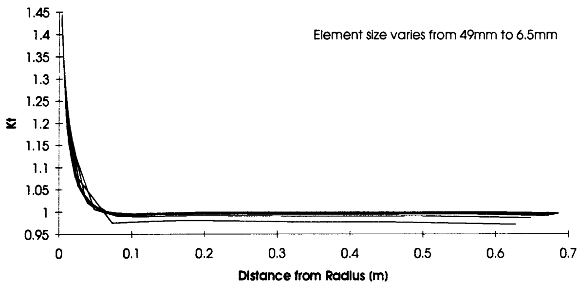
Figure 3.30: Stress Distribution along edge of plate (All Meshes)
