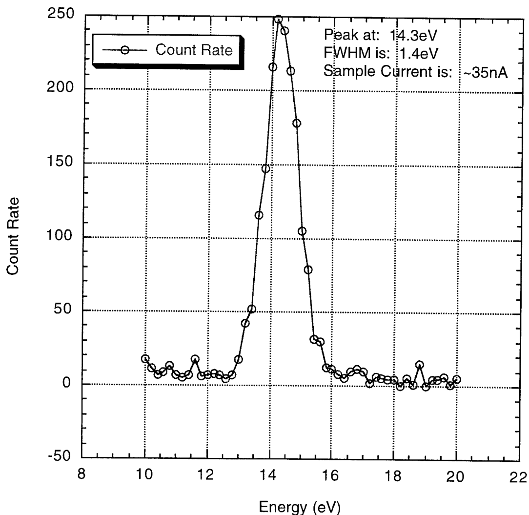
Figure 1. Energy distribution of Ga^+ ions from the Colutron ion source.
