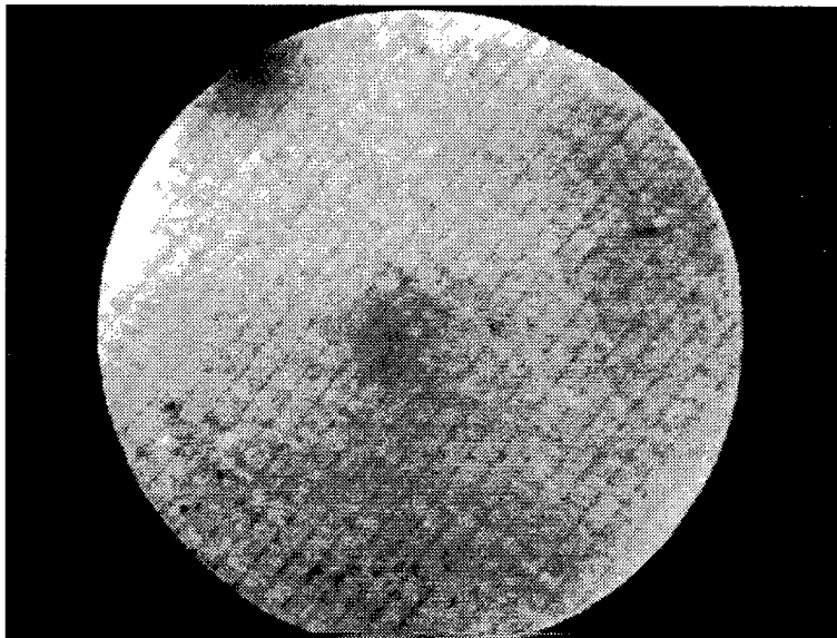
Figure 1. LEEM image of clean SiC surface. Energy 5.9 eV. Field of view 4.8 μm.
