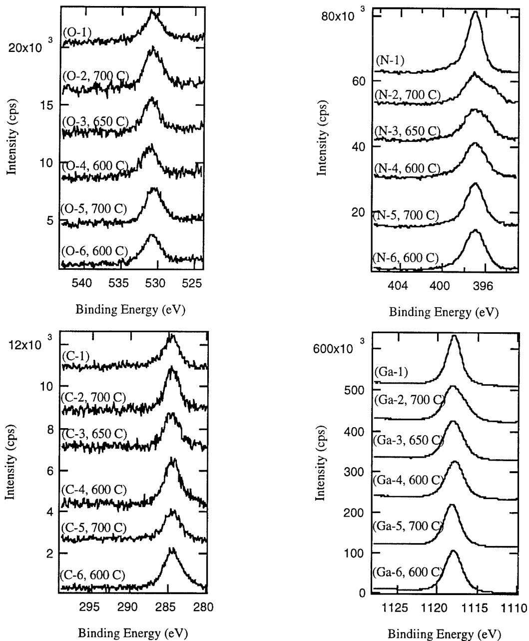
Figure 2. XPS spectra of samples after heat treatment at 800°C under NH 3 flux (1), after 3-h growth at 700°C (2), after 3-h growth at 650°C (3), after 3-h growth at 600°C (4), after 3-h growth at 700°C (5) and after 3-h growth at 600°C. NH 3 fluxes were 20 sccm for (2) through (4), and were 60 sccm for (5) and (6).
