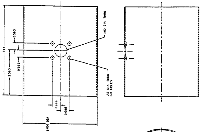
(17) COOLANT CHAMBER SHELL 93014F-07 SCALE: 1:1 MATERIAL: 304 S.S. MAX. THICK. 7/16 TYPE 304 STAINLESS STEEL
