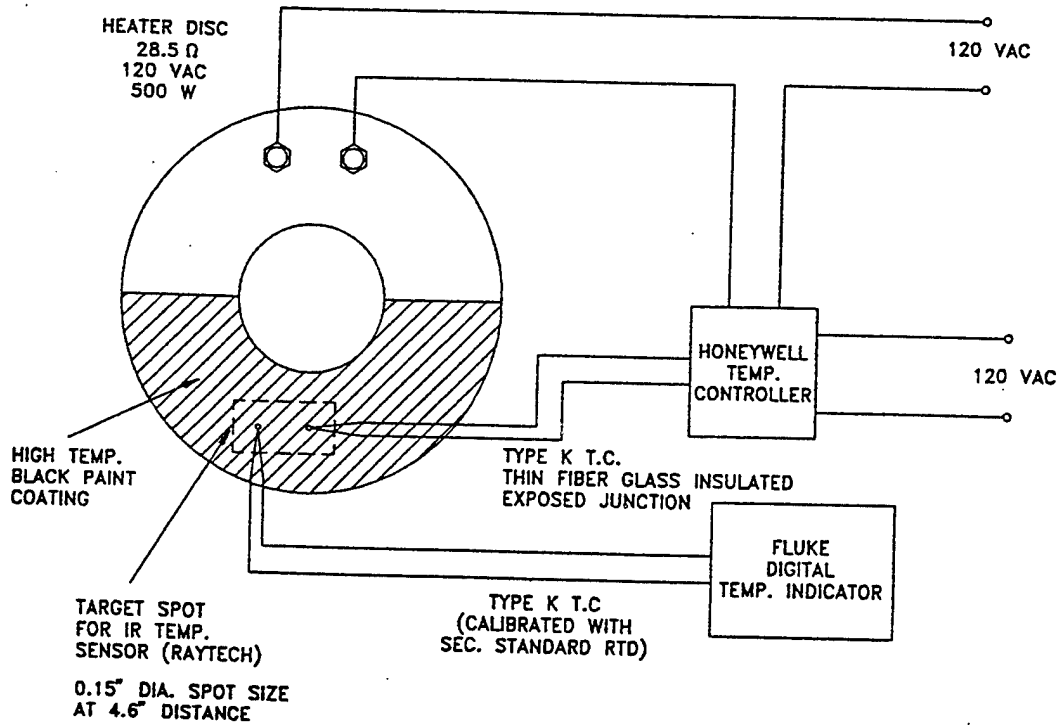
Figure 27. Calibration Source (0-300°C) for IR Sensor.
