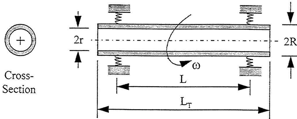
Figure A.5. RHP as a Simple Rigid Rotor in Flexible Supports.
