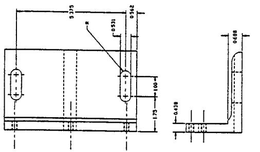
(29) COOLANT CHAMBER INLET MATERIAL: 4 x 4 x 1/2 ANGLE x 6 S/B 6061-T6 ALUMINUM
