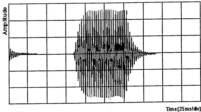
Y1420 (nominal 400 Hz resonance), loaded on forearm. Square wave modulation on 400 Hz carrier.
