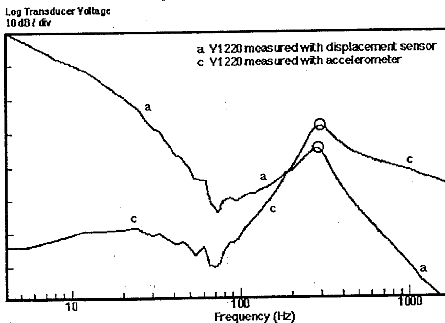
Frequency response for Y1220 (nom. 250 Hz resonance) transducer loaded on forearm
