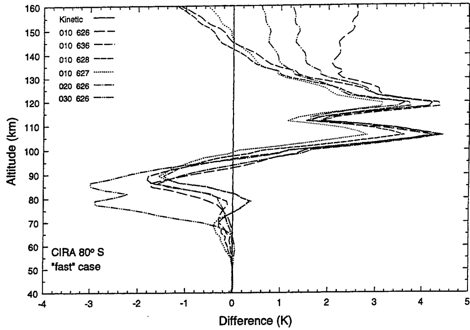
Figure 16. As Figure 12, but for the CIRA 80° S model atmosphere.
