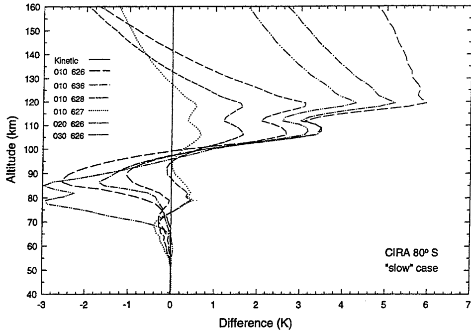
Figure 17. As Figure 16, but for the slow case.
