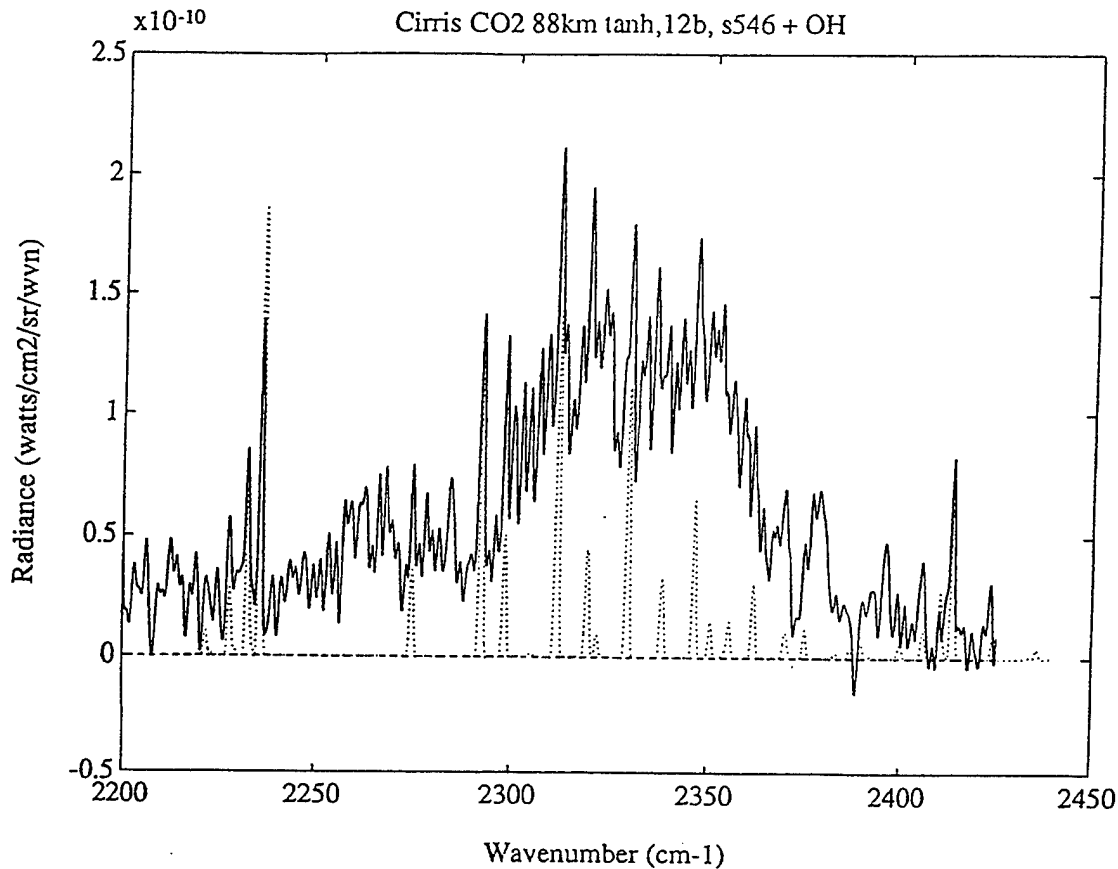
Figure 32. CIRRIS nighttime spectrum with tangent height at 88 km, with model results for OH lines superposed.
