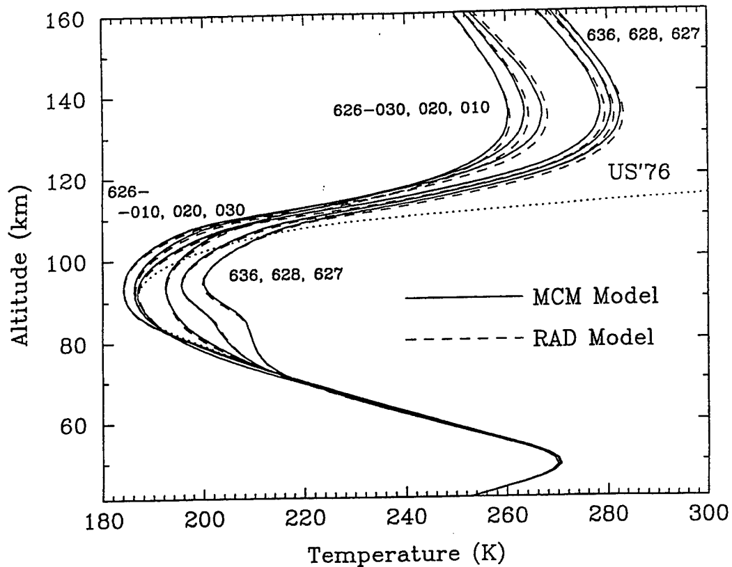
Figure 10. Comparison of MCM and RAD vibrational temperatures for the \text{CO}_2 01101 states for four isotopes, plus the 02201 and 03301 states for the major isotope. The calculations were performed with the larger oxygen-atom rate constant (the “fast” case; see text) using the smoothed U.S. Standard Atmosphere temperature profile
