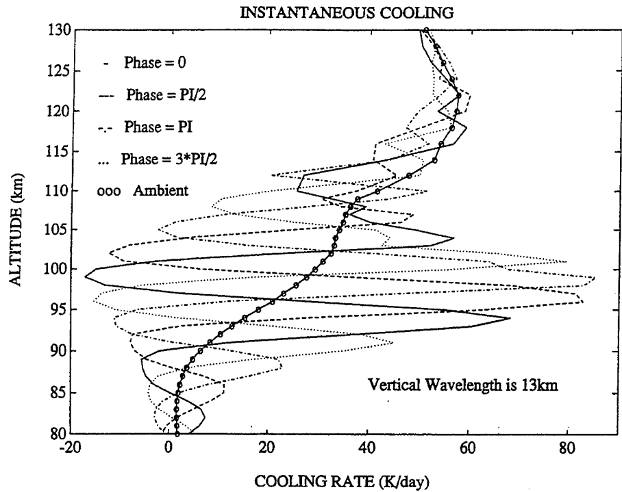
Figure 25. Instantaneous cooling due to the 15 \mu\text{m} bands, for four phases of the wave with the 13-km vertical wavelength.
