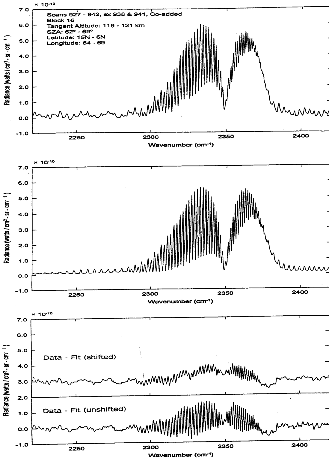
Figure 29a (top) CIRRIS data in the 4.3 \mu m region. Thirteen spectra were co-added; 29b (middle) Fit to the data in (a); 29c (bottom, top curve) Residuals from fit to the data in (a); 29d (bottom, bottom curve) Residuals from fit to the data in (a), with the wavenumber shift suppressed.
