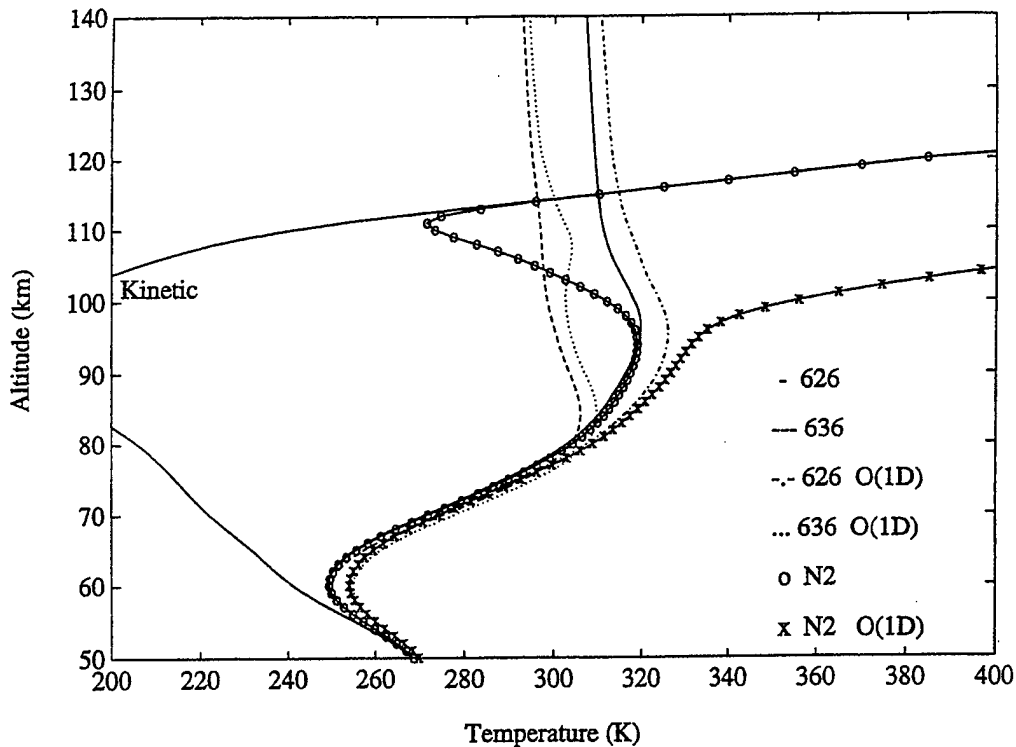
Figure 37. Vibrational temperatures of the CO 2 626 and 636 00011 state, and the N 2 (v=1) state, for a solar zenith angle of 2.2°, calculated with and without the O( 1 D) excitation mechanism.
