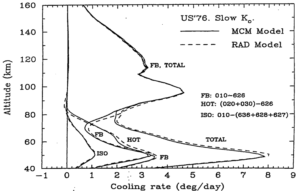
Figure 19. Comparison of the total cooling due to 15 \mu\text{m} emission as calculated by MCM and RAD for the mid-latitude model and the slow case. Contributions from the 626 fundamental band, the minor-isotope fundamentals, and the hot bands are also shown.
