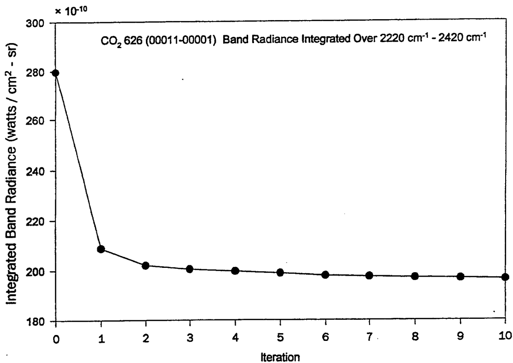
Figure 28. Convergence of iterative fitting algorithm for CO 2 (ν 3 ) fundamental band.
