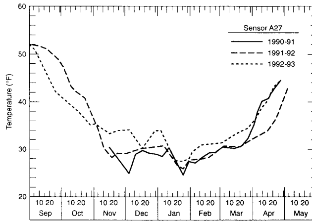
Figure 18. Yearly temperatures under horizontal ground insulation.
