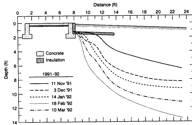
Figure 13. Isotherm (32°F) for the winter of 1991-92.
