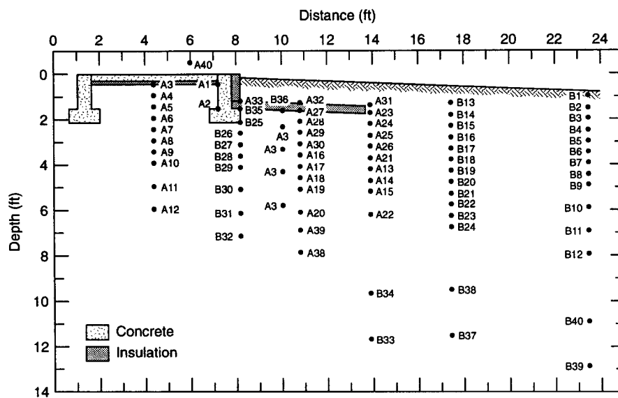
Figure 5. Location of temperature sensors.
