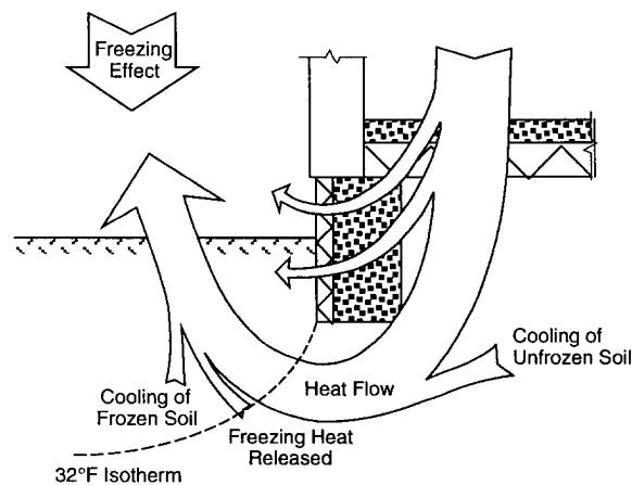
Figure 3. Heat flow lines around a shallow insulated foundation.
