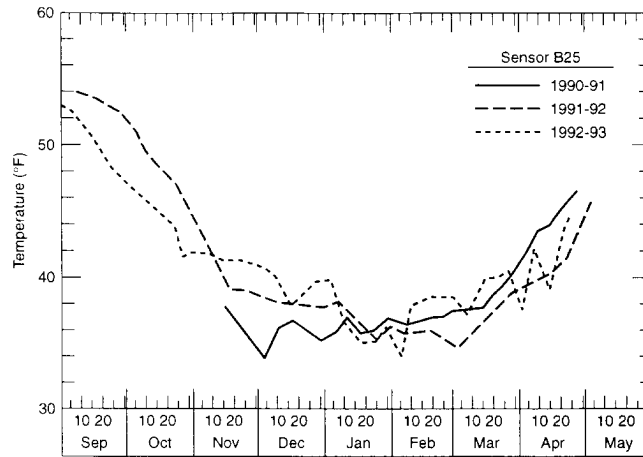
Figure 17. Yearly temperatures at toe of footing.
