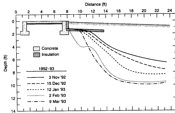
Figure 14. Isotherm (32°F) for the winter of 1992-93.
