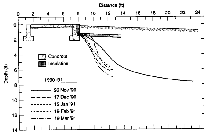
Figure 12. Isotherm (32°F) for the winter of 1990-91.
