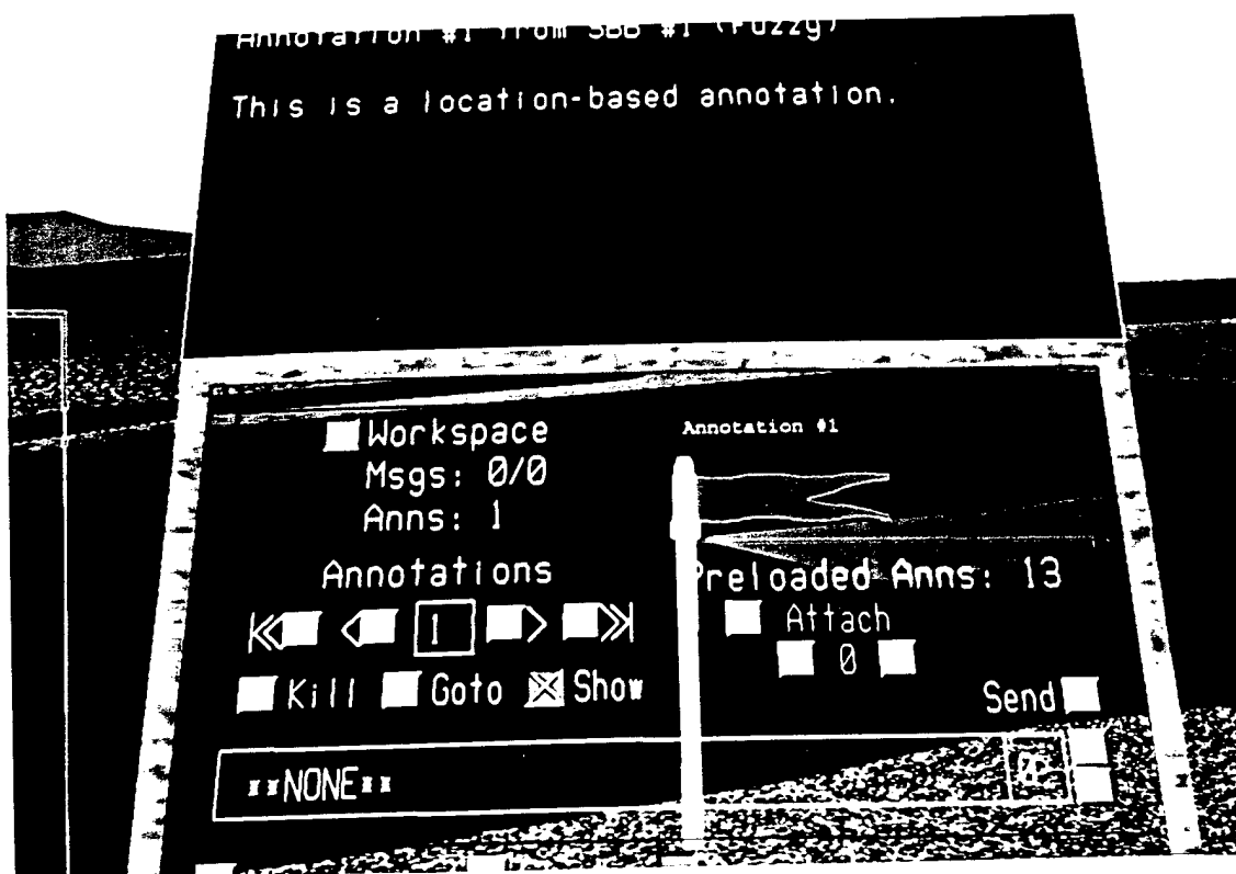
Figure 4-18. Old Annotation.
