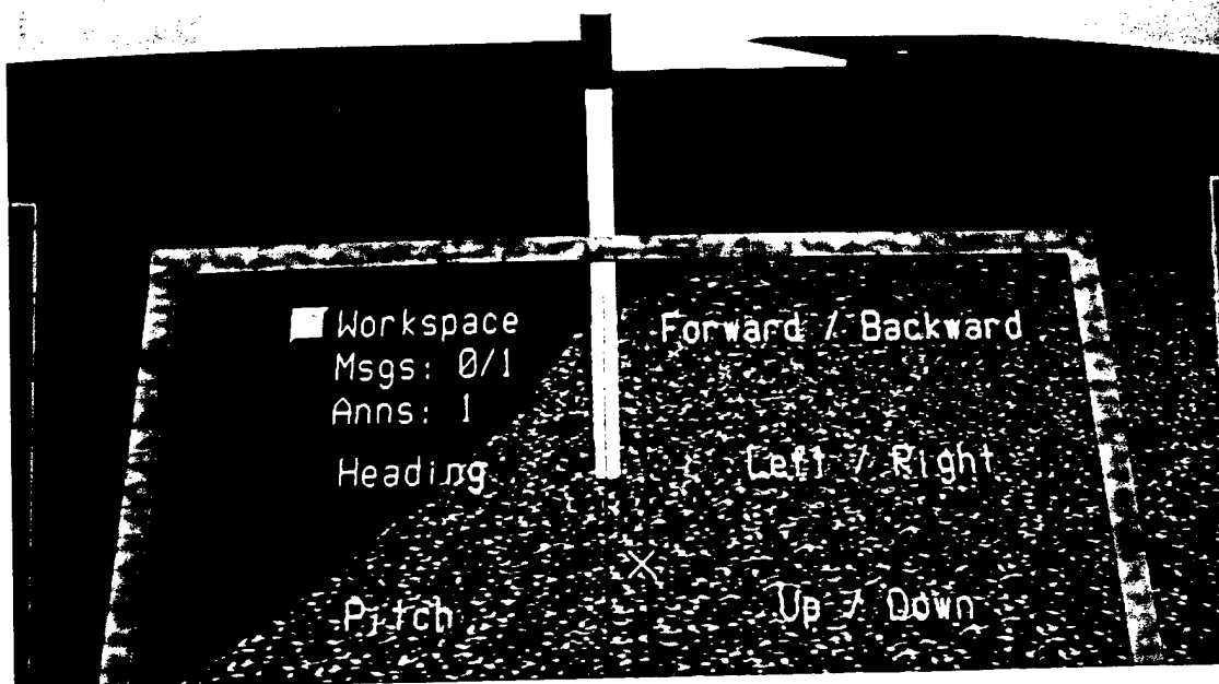
Figure 4-17. Selected Annotation.
