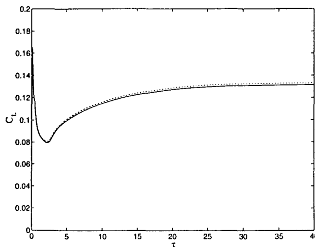
Fig. 1 Lift response vs time for a NACA 0012 airfoil at Mach 0.5 and zero angle of attack, subjected to a 1-deg step change in angle of attack: ST code (—), linearized ST code (---), \epsilon_e = 2 , \epsilon_i = 0 and \Delta\tau = 0.004 .
