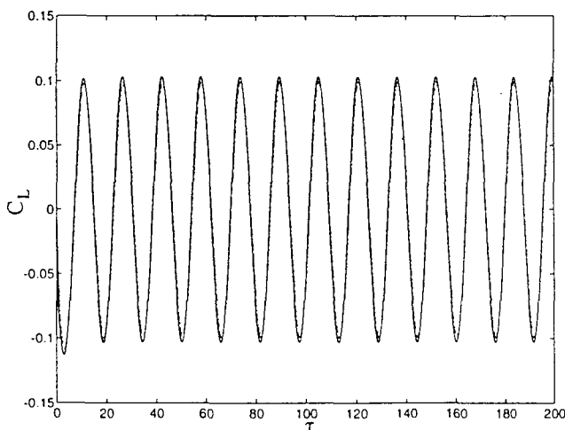
Fig. 4 Lift response vs time for a NACA 0012 airfoil at Mach 0.5 oscillating at \pm 1 deg about zero angle of attack; k = 0.4 , coarse mesh, \epsilon_r = 2 , \epsilon_i = 0 , \Delta\tau = 0.004 ; linearized ST, and 100 modes overlay (---), 50 modes (—), 10 modes (···).
