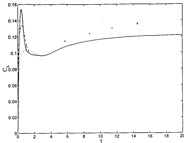
Fig. 2 Lift response vs time for a NACA 0012 airfoil at Mach 0.5 and zero angle of attack, subjected to a 1-deg step change in angle of attack; coarse mesh, \epsilon_r = 2 , \epsilon_i = 0 , \Delta\tau = 0.004 , linearized ST, all modes, and 200 modes overlay (---), 100 modes (—), 50 modes (···).
