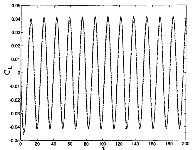
Fig. 5 Lift response vs time for a NACA 0012 airfoil at Mach 0.5 in plunging oscillation; h/c = 0.01 , k = 0.4 , coarse mesh, \epsilon_r = 2 , \epsilon_i = 0 , \Delta\tau = 0.004 ; linearized ST and 50 modes overlay (---), 10 modes (—), 1 modes (···).
