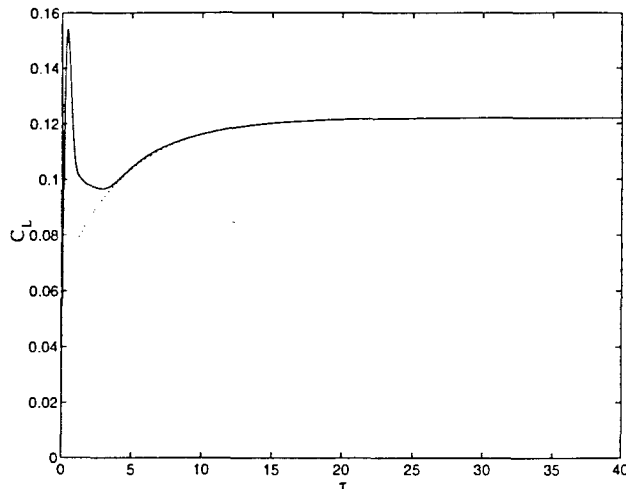
Fig. 3 Lift response vs time for a NACA 0012 airfoil at Mach 0.5 and zero angle of attack, subjected to a 1-deg step change in angle of attack; coarse mesh, \epsilon_r = 2 , \epsilon_i = 0 , \Delta\tau = 0.004 , linearized ST (—), 1 mode (···).
