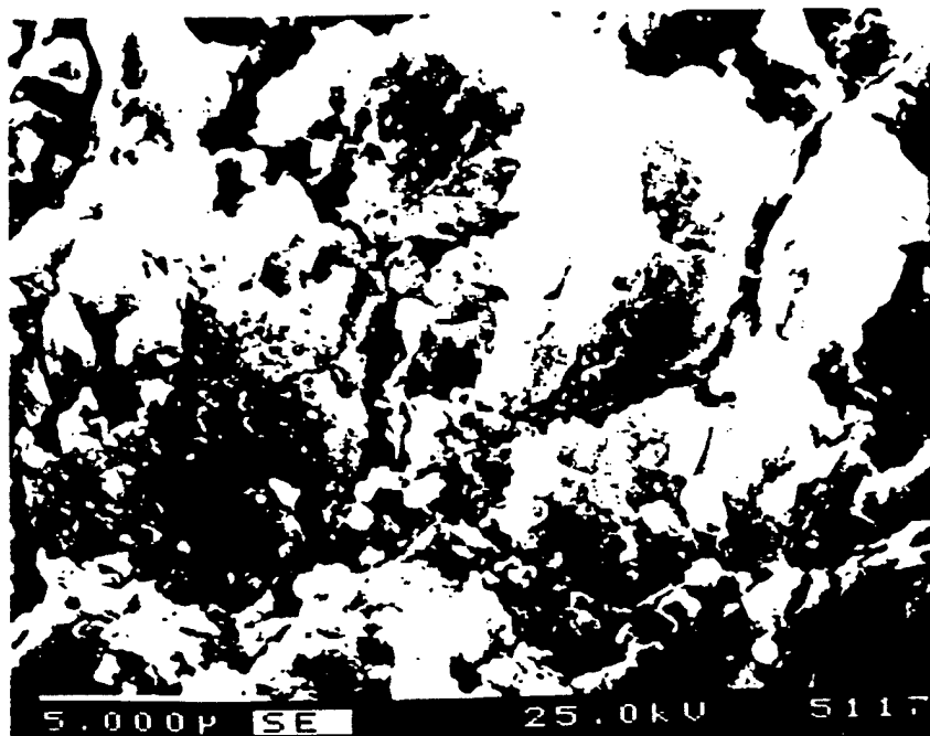
Figure 9-11. SEM morphology of Zircadyne 702, showing structure of ZrO 2 scale after oxidation in 5 wt.% Hcl solution at 450°C, 30 min.
