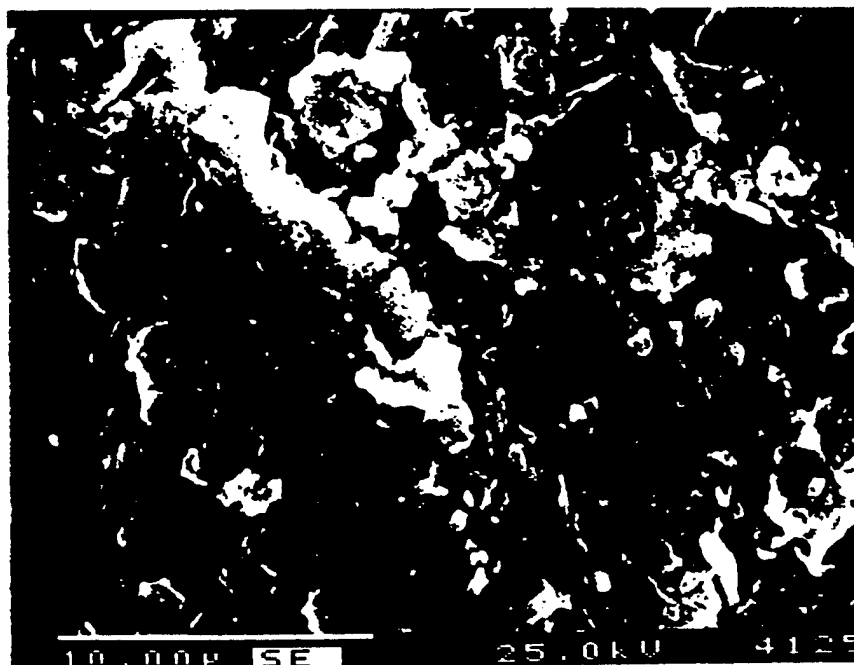
Figure 9-12. SEM morphology of Zircadyne 705, showing structure of ZrO 2 scale after oxidation in 5 wt.% Hcl solution at 450°C, 30 min.
