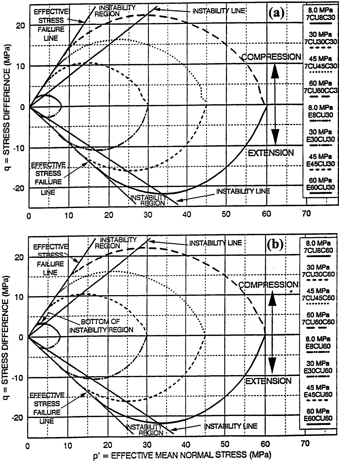
Fig. 3. Instability lines and failure lines determined from consolidated-undrained triaxial compression and extension tests on Cambria sand with initial relative densities of (a) 30%, and (b) 60%.
