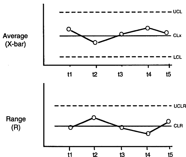
Figure 5-4: X-Bar and Range Charts for a Process That Is in Control
