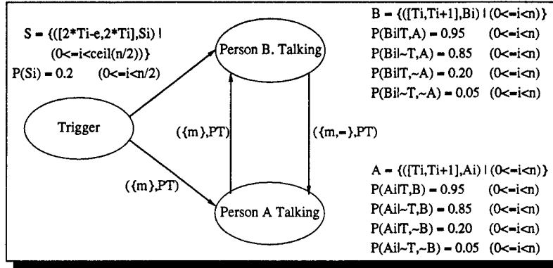
Figure 11: PTN modeling two people chatting with an occasional conversational trigger. Note the use of set-builder notation.
