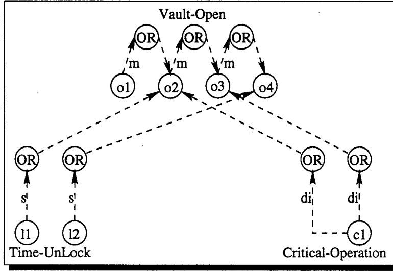
Figure 9: Expanded Probabilistic Temporal Network for PTN in Figure 3. Labels on arcs indicate temporal relation; during inverse, starts, meets.
