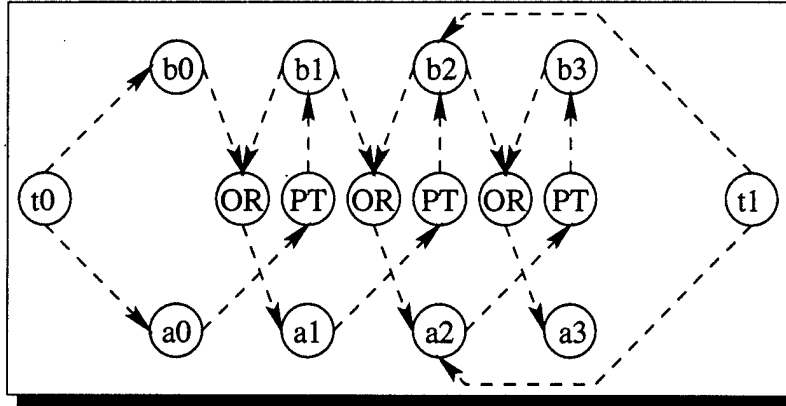
Figure 12: EPTN for PTN in Figure 11 with n = 4 .
