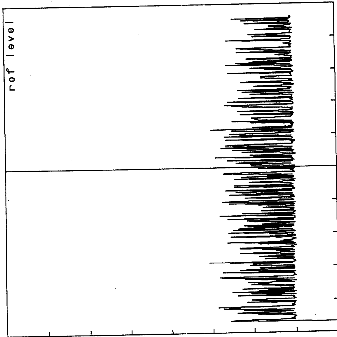
Fig 4b Spectrum of discharge
