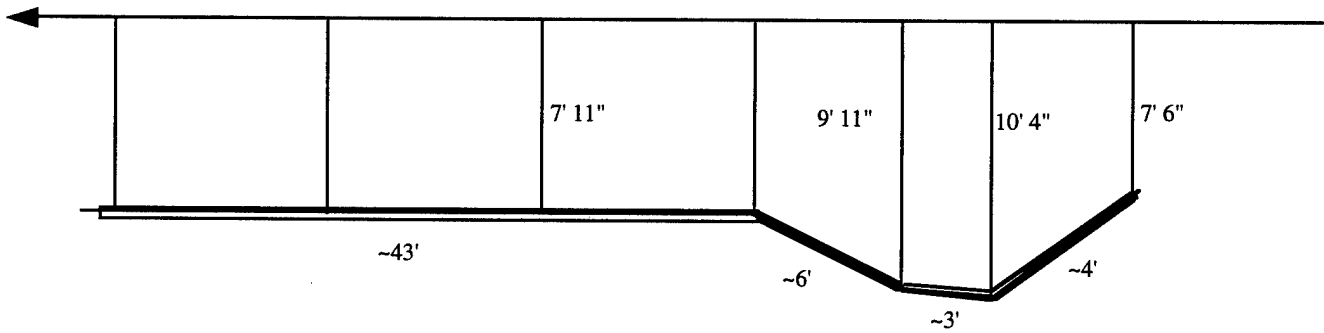
Figure 4. Continuous Line Charge Arrangement at Varying Depths
