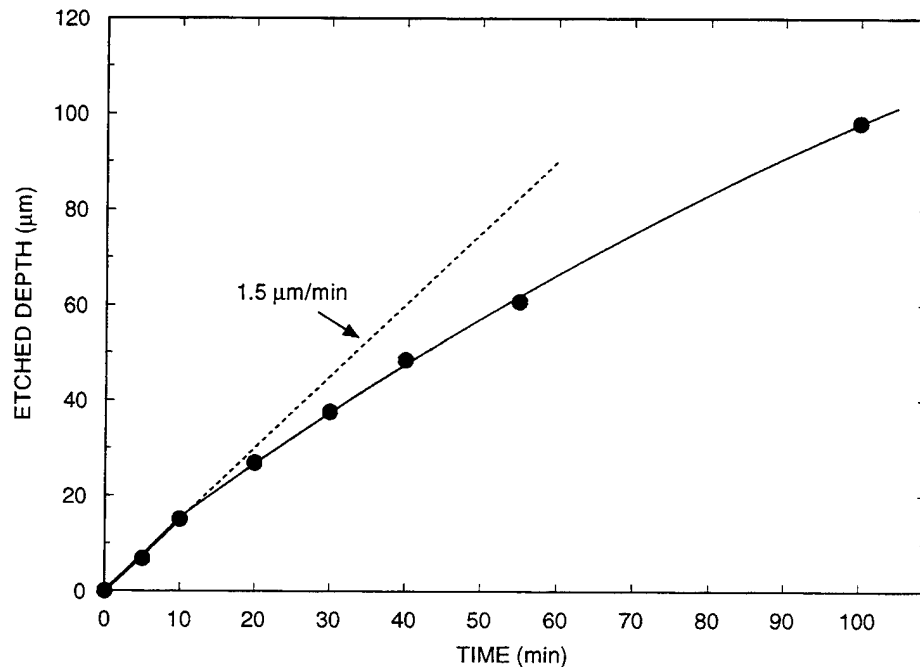
Figure B-1. Etched depth versus time for Ag foil SUB42 etched by a 3:1:44 molar ratio of \text{KI}:\text{I}_2:\text{H}_2\text{O} . The initial etch rate is indicated by the dashed line. The solid line is a guide to the eye.
