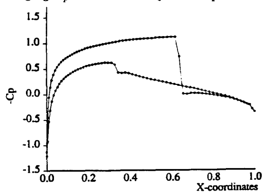
Fig.3h C_p distribution by consistent-mass
