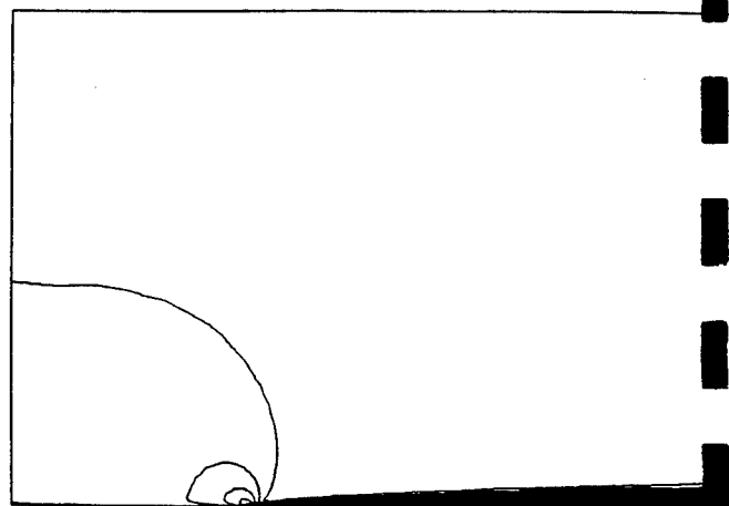
Fig.2b Computed Mach Number Contours past a Flat Plate; M_\infty = 0.5 , Re=10,000
