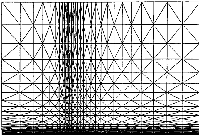
Fig.2a Mesh Used for Computing Viscous Flow past a Flat Plate; nelem=2,604 , npoin=1,376
