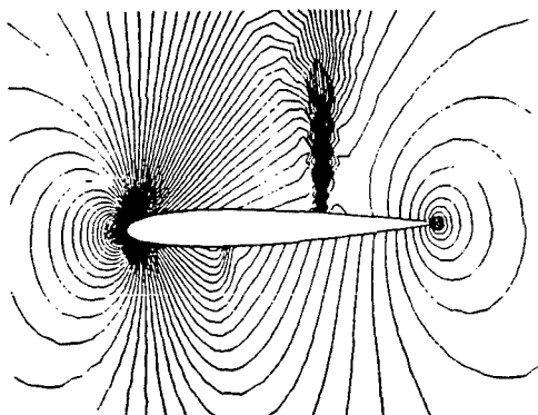
Fig.3c Pressure contours by least-squares
