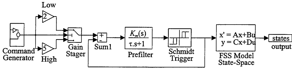
(a) Open Loop PWWF Simulation
