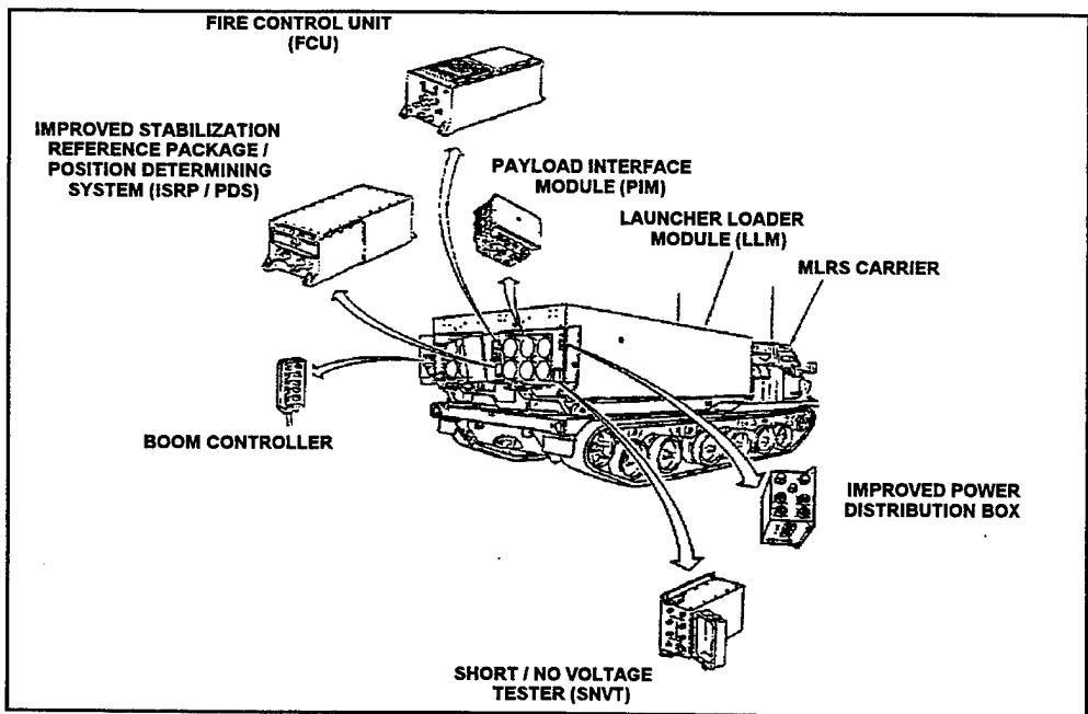
Figure 1-3 M269 Mounted LRUs [Ref. 2, p.14]
