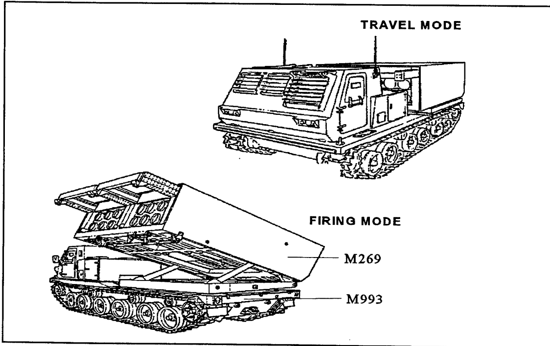
Figure 1-1 MLRS Configuration Modes M270 [Ref. 2, p. 2]
