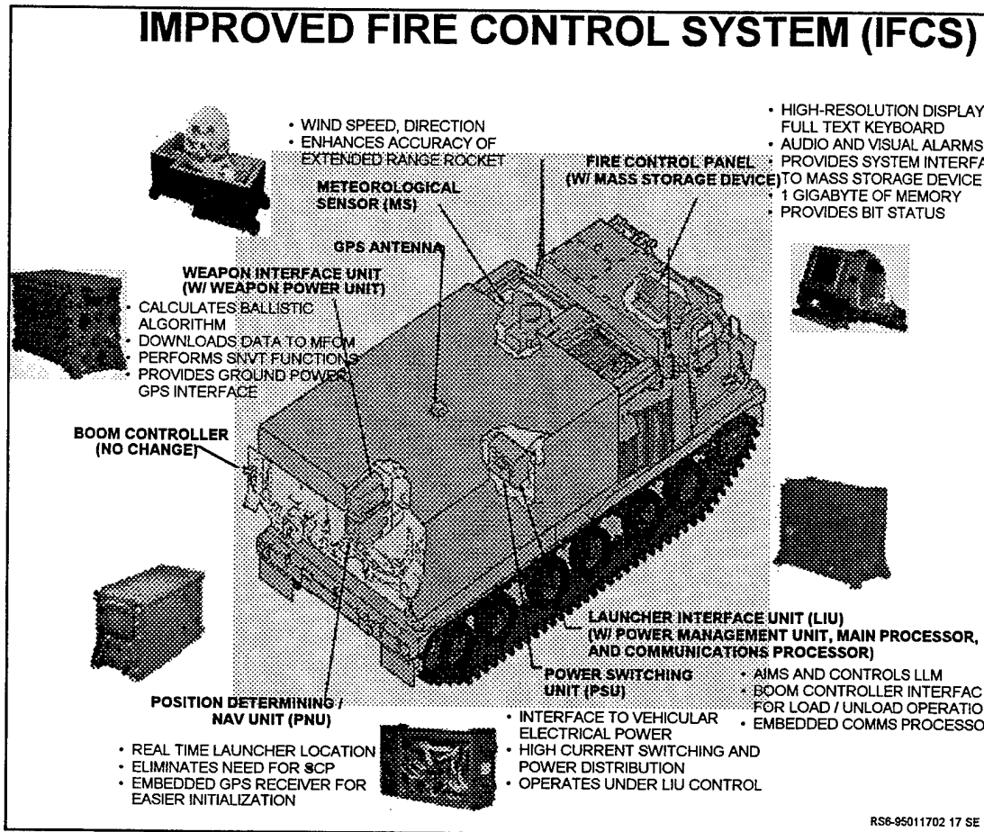
Figure 1-4 IFCS [Ref. 2, p. E- 13]
