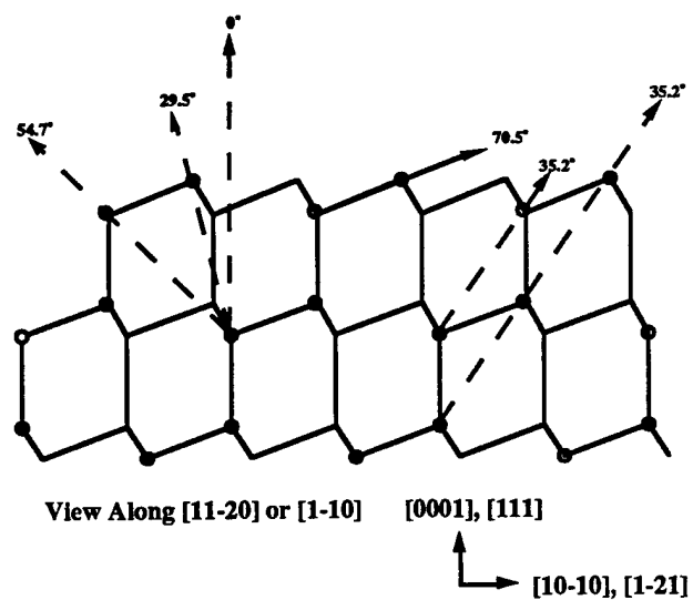
Figure 13. Schematic illustrating expected forward scattering/focusing peaks in XPD along the [11-20] azimuth of 3C/6H-SiC.
