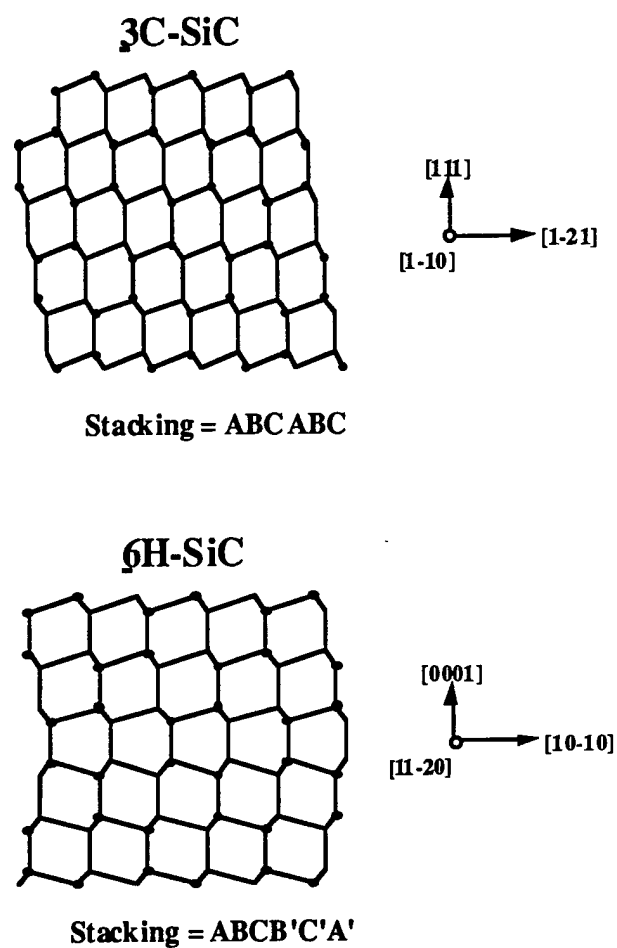
Figure 12. Schematic illustrating the differences in stacking along the [111]/[0001] direction for 3C and 6H-SiC.
