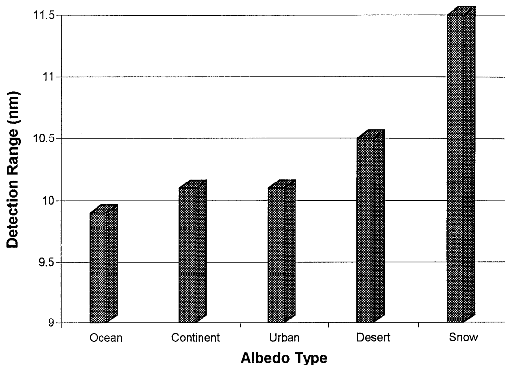
Figure 30. Detection range versus albedo type on 10 Jan 96/0300Z for bunker target.
