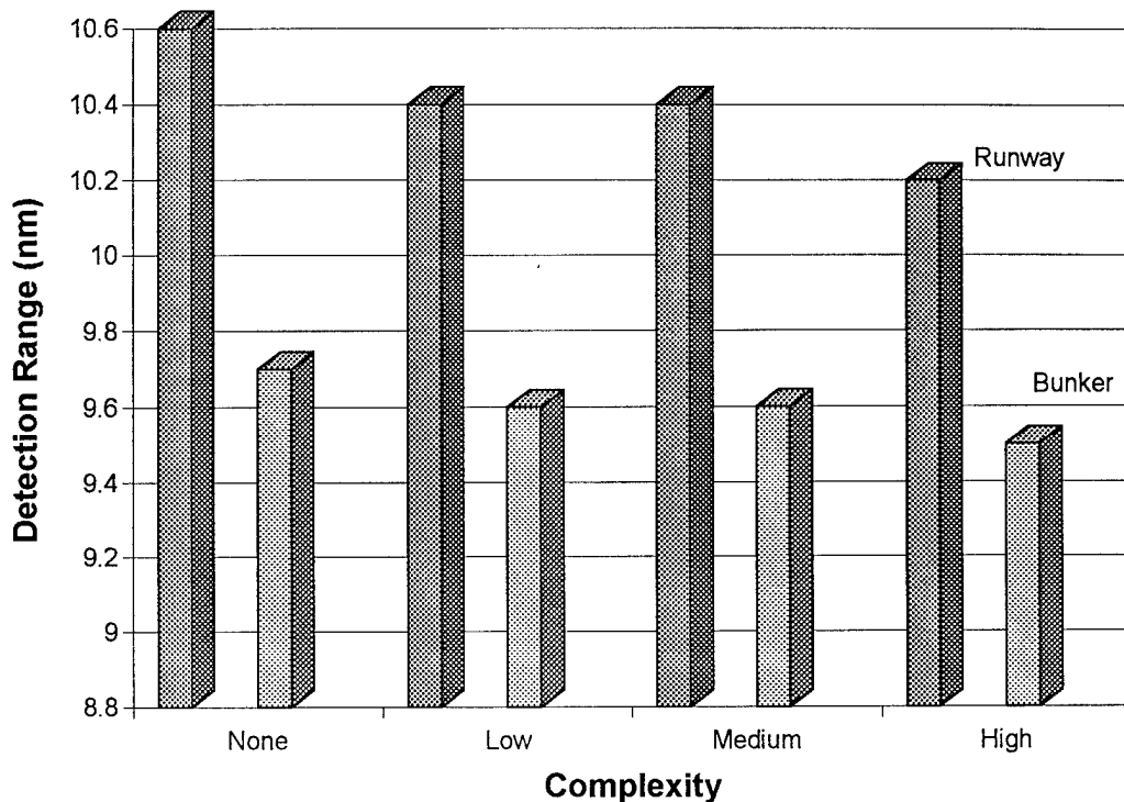
Figure 27. Detection range versus target scene complexity on 10 and 20 Jan 96 with the bunker and runway targets, respectively.
